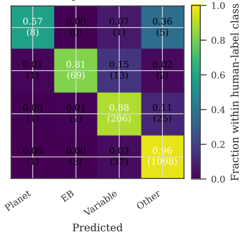
(b) Primary: all real test labels
