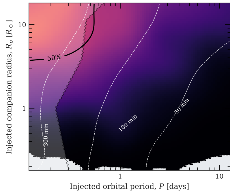
18 <= Tmag < 19: 485/1796 recovered
