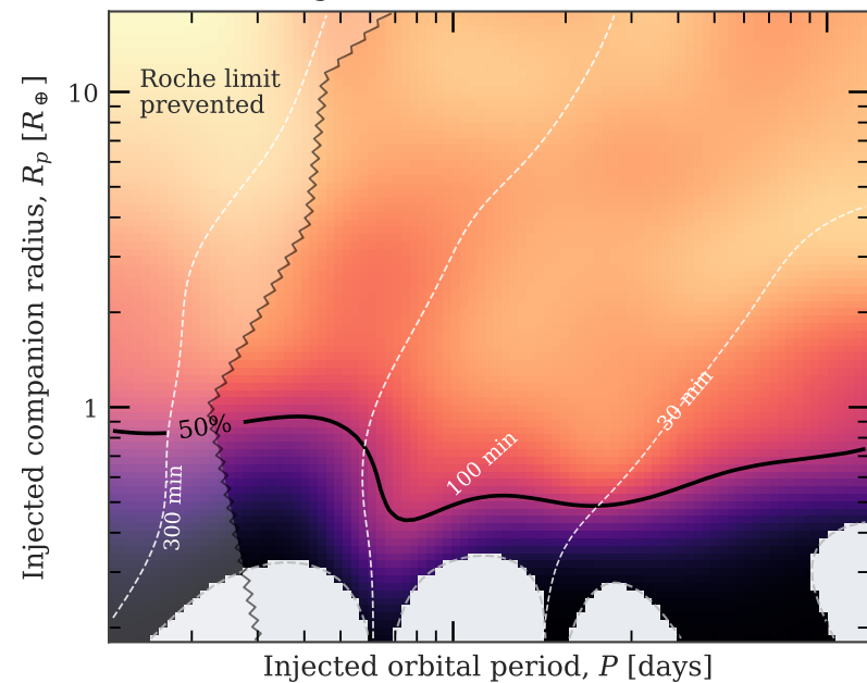
Tmag < 17: 218/275 recovered
