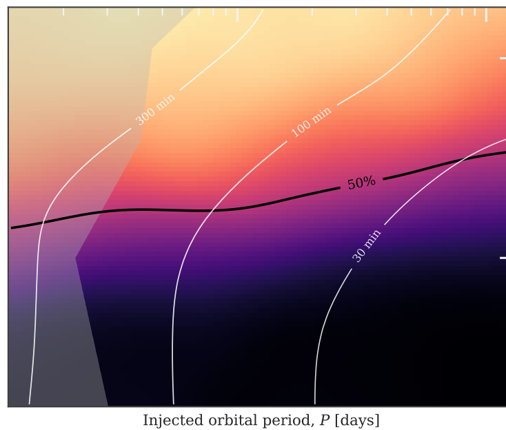
17 &lt;= Tmag &lt; 18: 2273/4994 recovered
