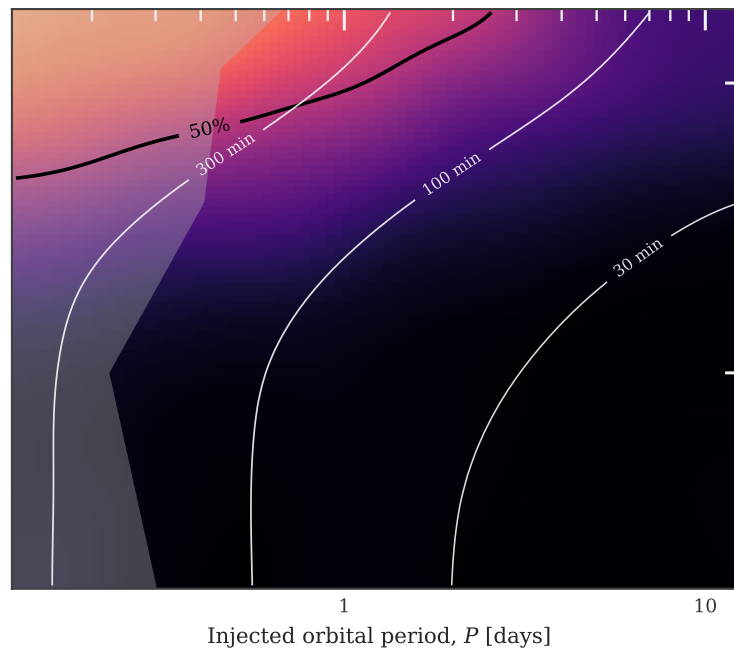
Tmag &gt; 19: 858/4960 recovered
