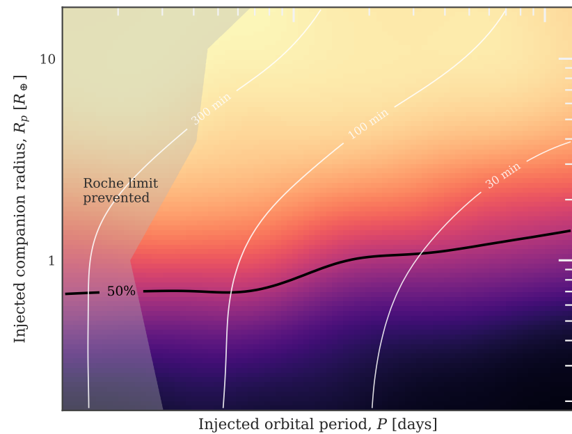
Tmag &lt; 17: 3154/5020 recovered
