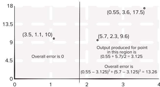
Regions and Errors Associated with x_1 < 1.8
