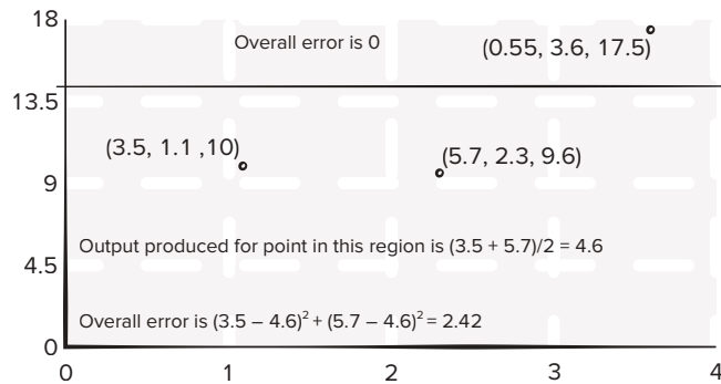
Regions and Errors Associated with x_2 < 15
