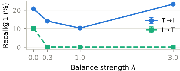
(a) MSCOCO: T \rightarrow I non-monotonic, I \rightarrow T collapses
