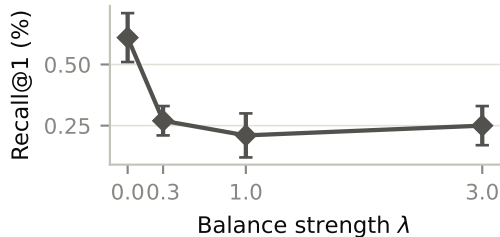
(b) FashionIQ: vanilla wins, any regularization hurts
