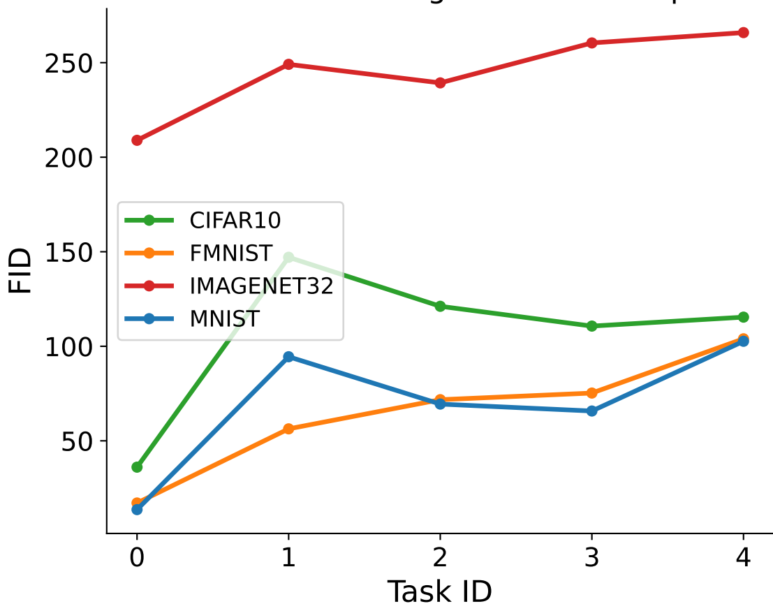
Non-continual Learning - Dataset Comparison
