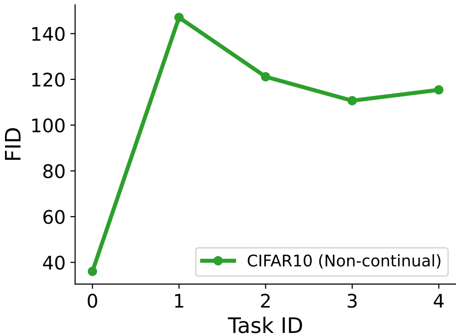
CIFAR10 - Non-continual
