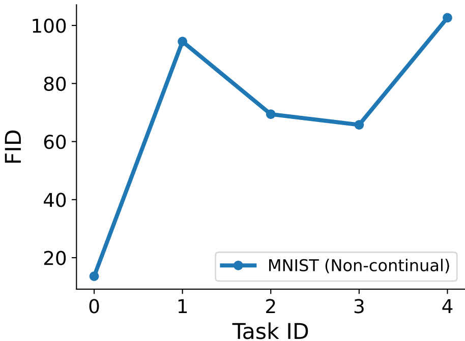
MNIST - Non-continual
