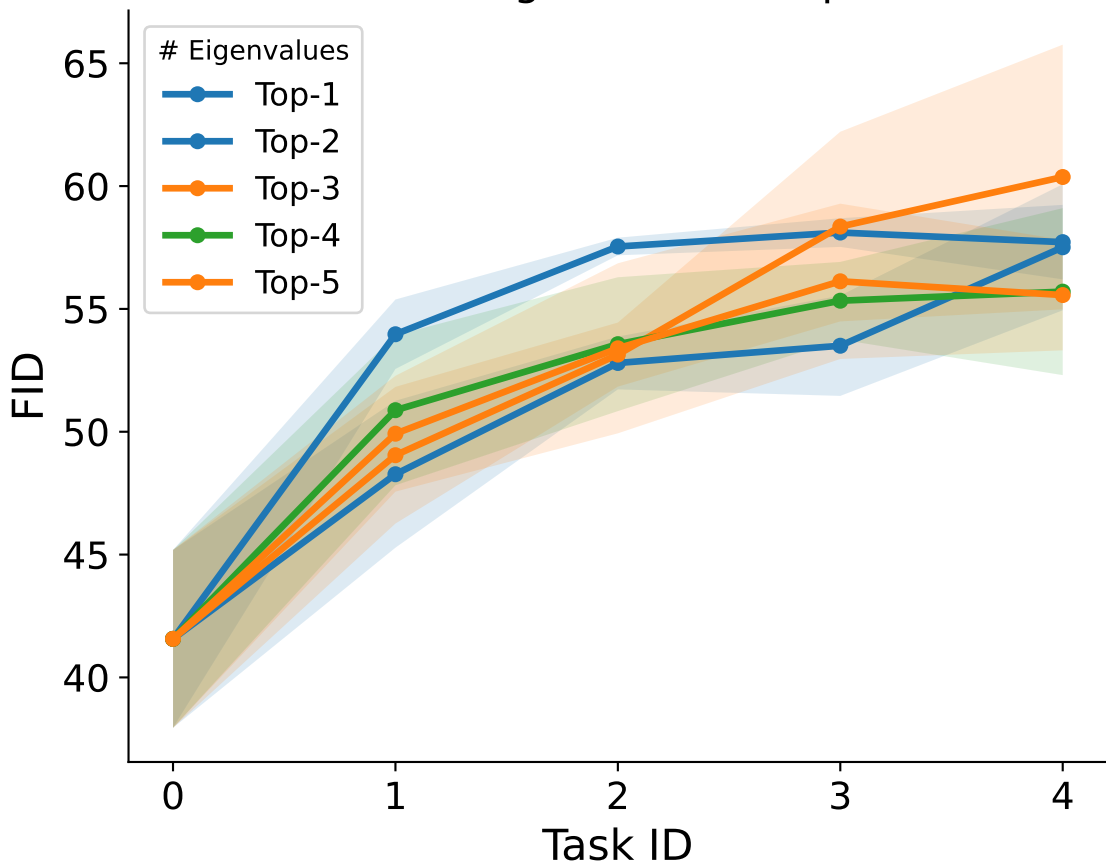
CIFAR10 - Eigenvalue Comparison
