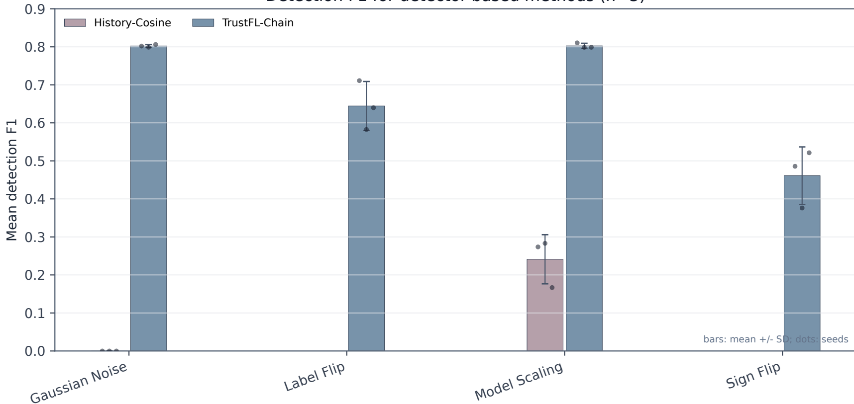
Detection F1 for detector-based methods (n=3)
