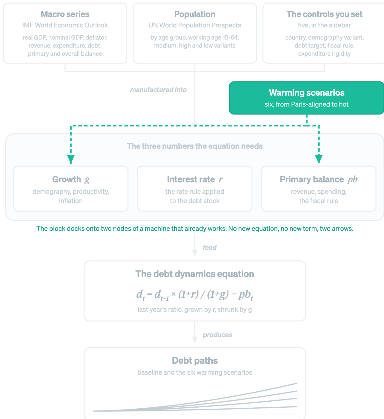
Figure 6.3: Step 3 adds one block and two arrows. The equation is untouched, the sources are untouched, and the interest rate never hears about the weather.
