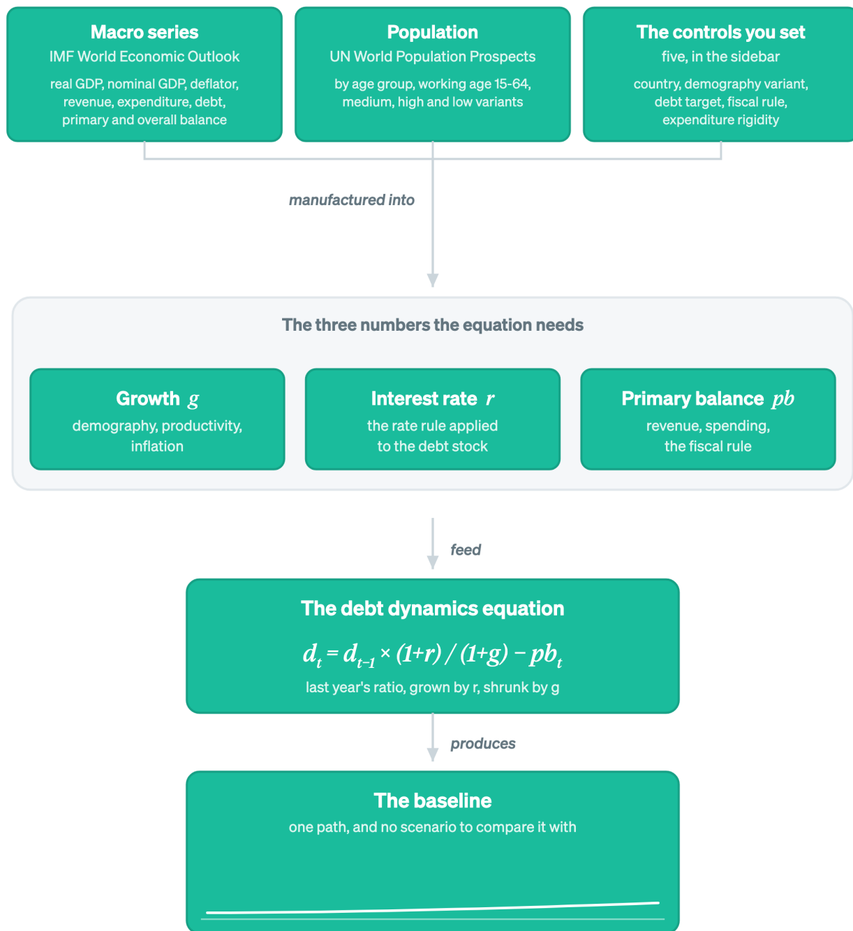
Figure 5.5: The end of Step 2: a complete long-term fiscal projection model. The warming block is not missing from this drawing, it has not been built yet. Run this chain and you get the baseline.
