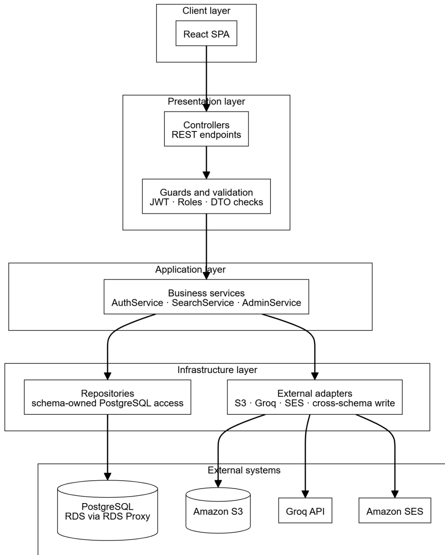
Figure 25: component diagram (Layering)
