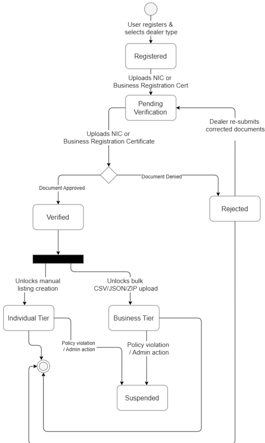
Figure 23: displays the state progression of a Dealer account within the Auth-User Service schema, illustrating the tiered onboarding process. An account begins as REGISTERED and moves to PENDING_VERIFICATION once required documentation is uploaded to S3. An Administrator reviews these documents. Approved documents transition the account to a VERIFIED state, unlocking specific capabilities based on the dealer tier (capped manual listings for Individual, bulk ingestion for
