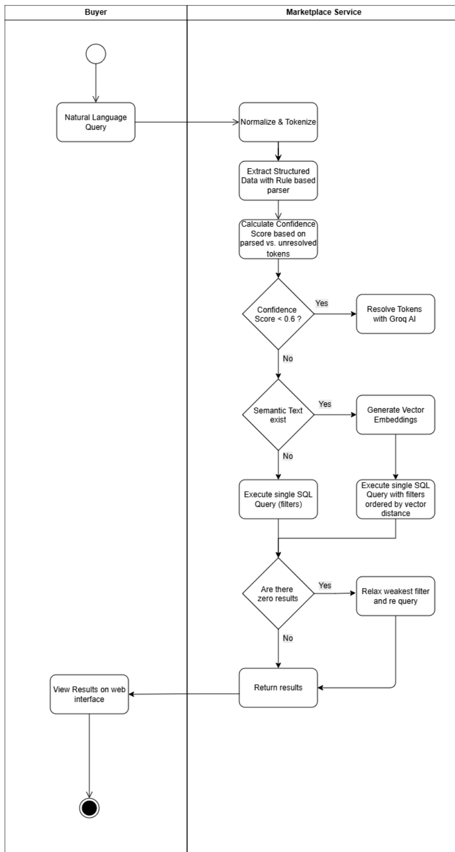
Figure 18: describes how a buyer's free-text query is processed by the Marketplace Service. The query is tokenized and passed through a multi-stage deterministic parser that extracts multi-word
