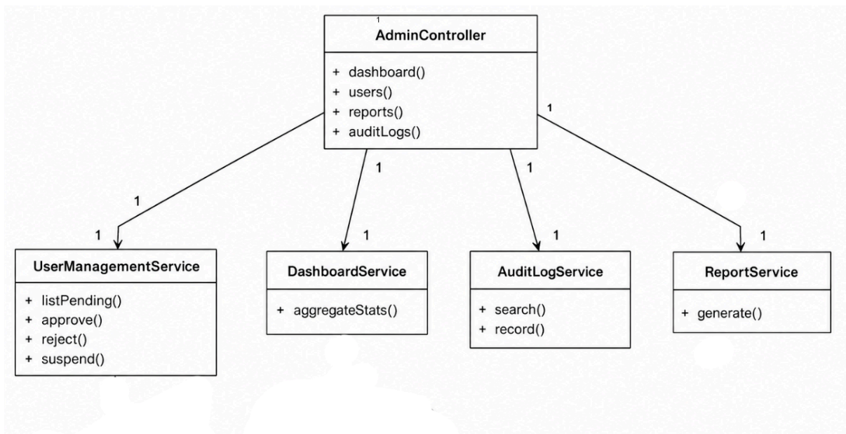
Figure 15 : Admin class diagram
