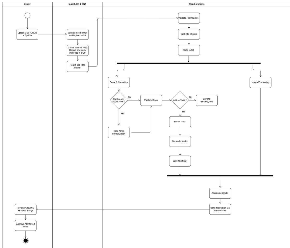
Figure 17: shows the end-to-end workflow of bulk inventory upload from the perspective of the Dealer, Ingest API, AWS Step Functions, and SQS swimlanes. The dealer uploads a CSV or JSON file that contains data about vehicles together with a ZIP file of vehicle images. As the aim is to provide a synchronous response at a rapid pace, the Ingest API only runs a lightweight validation, keeps the files unmodified in the S3 storage service of Amazon, and kicks off an SQS queue with a message.
