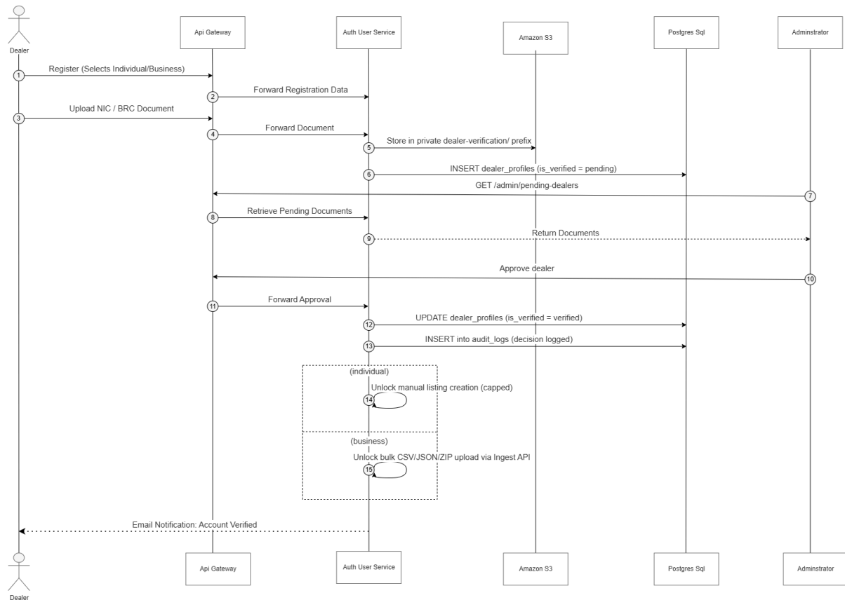
Figure 19: shows how the registration, validation, and authorization for a Dealer are accomplished via the Auth-User service. During registration, the dealer is required to enter a dealer type, which can be either Individual or Business, and provide the required supporting document, which can be NIC and/or Business Registration Certificate. The provided documents are stored in a private bucket on Amazon S3.
