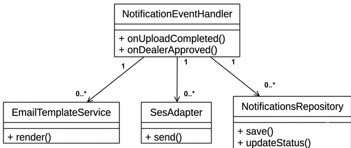
Figure 16: Notification class diagram
