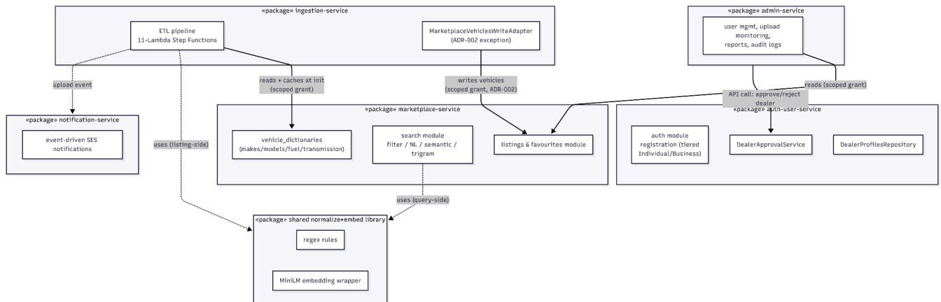
Figure 11 : Backend module packages and documented cross-module dependencies (shared RDS, modular monolith).
