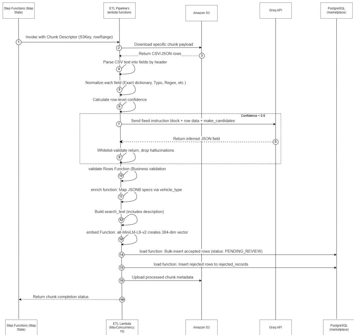
Figure 21: represents the Parallel Data Processing Loop in the AWS Step Functions Map State. Due to limitations set by AWS payload size, the state machine operates on an execution-per-upload basis. The SplitIntoChunks step results in a small array of descriptors pointing to row ranges in S3, which is spread out using the Map state up to 10 concurrent executions in order to keep the database connection pool safe.
