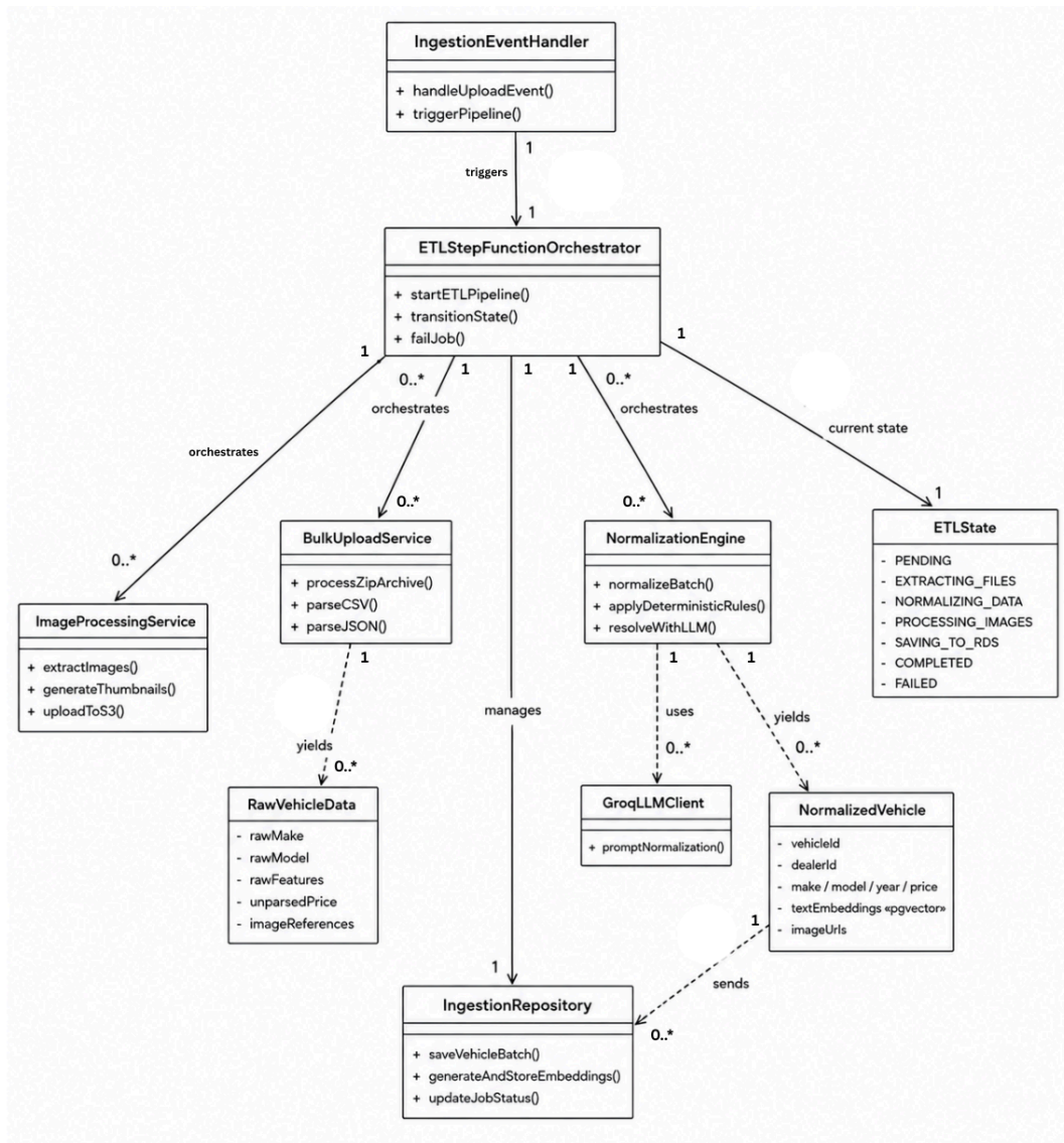
Figure 14 : Ingestion class diagram
