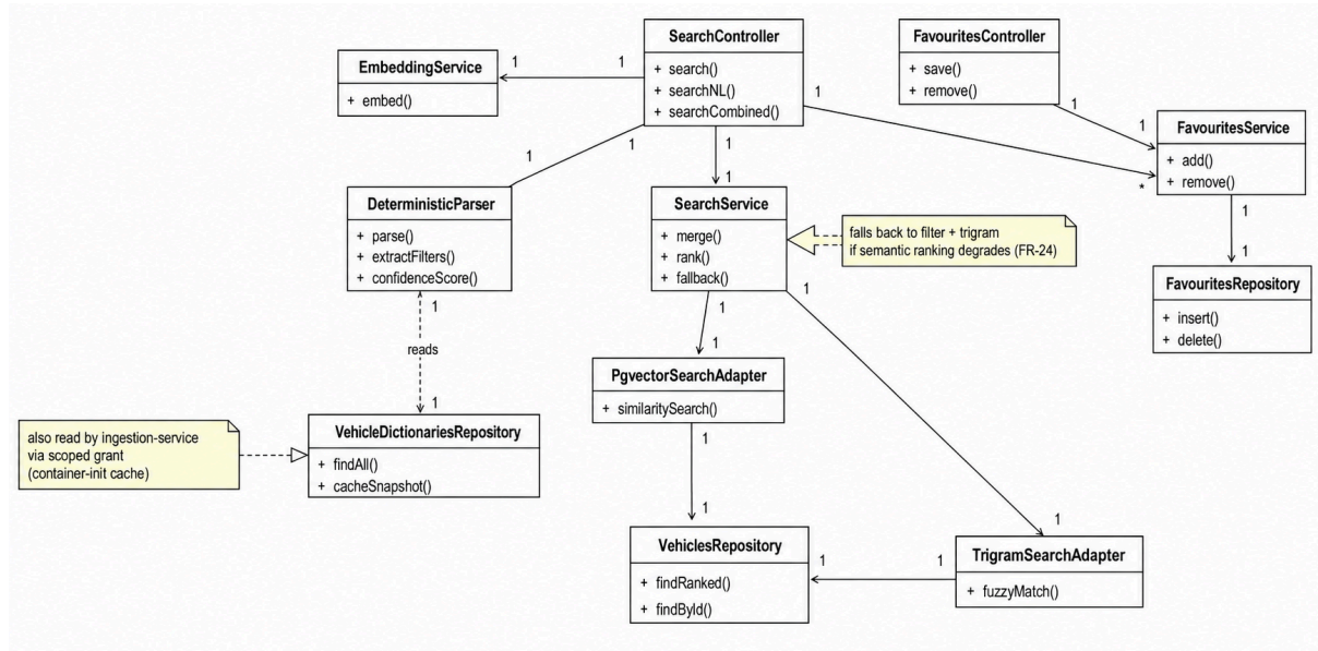
Figure 13 : Marketplace class diagram
