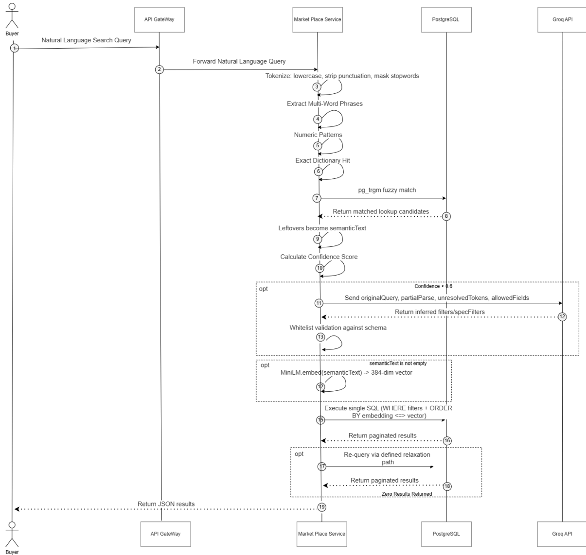
Figure 22: presents the execution flow of a natural-language search query processed by a deterministic 5-stage parser. The tokenizer lowercases text, strips punctuation, splits words, and masks domain-specific stopwords without deleting them. The parser extracts multi-word phrases and numeric patterns, flagging adjacent tokens as digit-adjacent. It then executes exact dictionary hits, strictly resolving Make before Model. Stage 4 performs fuzzy matching using pg_trgm for large vocabularies, utilizing type-gating to reject digit-adjacent tokens outright. Unconsumed tokens are routed into semanticText.
