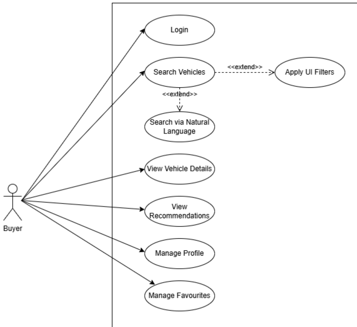
Figure 8 : the functions available to a buyer. The "Manage Favourites" and "View Recommendations" use cases have significant architectural coverage, as they bridge authentication boundaries, require foreign-key interactions between the auth and marketplace database schemas, and heavily utilize semantic similarity calculations.
