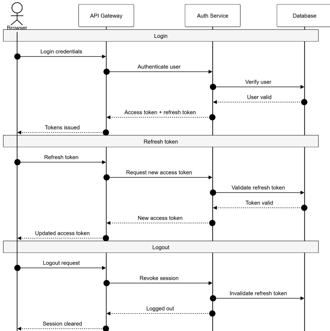
Figure 02: Authentication sequence - login, refresh, and logout. The browser sends credentials to the Auth Service via the API Gateway. On success, short-lived access tokens and longer-lived refresh tokens are issued. Refresh tokens are validated server-side and can be revoked on logout.
