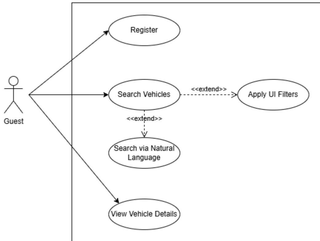
Figure 7 : shows the main functions available to an unauthenticated guest. The architecturally significant guest function is the natural-language vehicle search, as it triggers the 5-stage deterministic parser, interacts with the external Groq LLM API for fallback resolution, and queries persistent vector embeddings using PostgreSQL's pgvector
