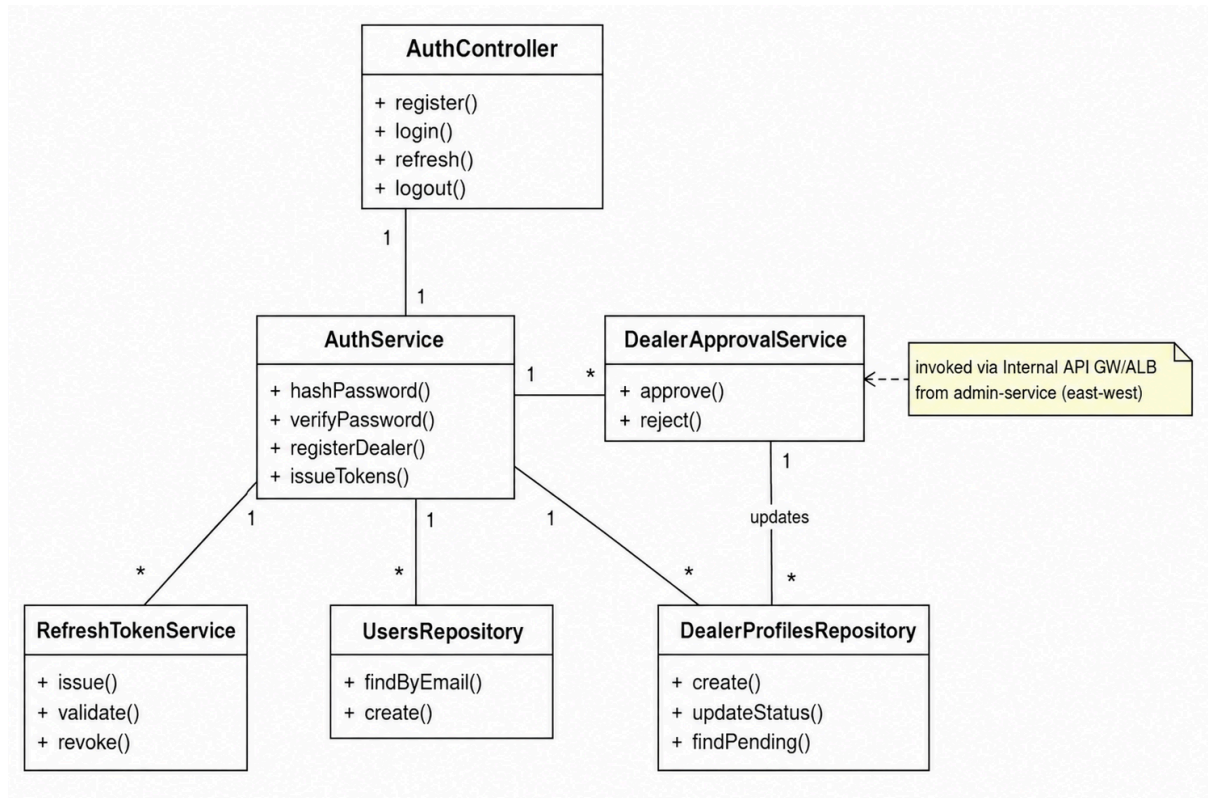
Figure 12: auth- user class diagram
