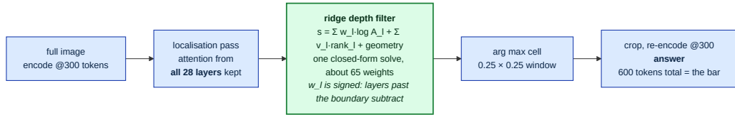
Figure 2: Policy I, the ridge depth filter. One localisation pass, every layer’s attention kept, a single closed-form solve that re-weights depths, and a crop. Nothing is selected: all 28 layers enter the score, and the fitted weights are signed, so layers past the transport boundary subtract rather than add.
