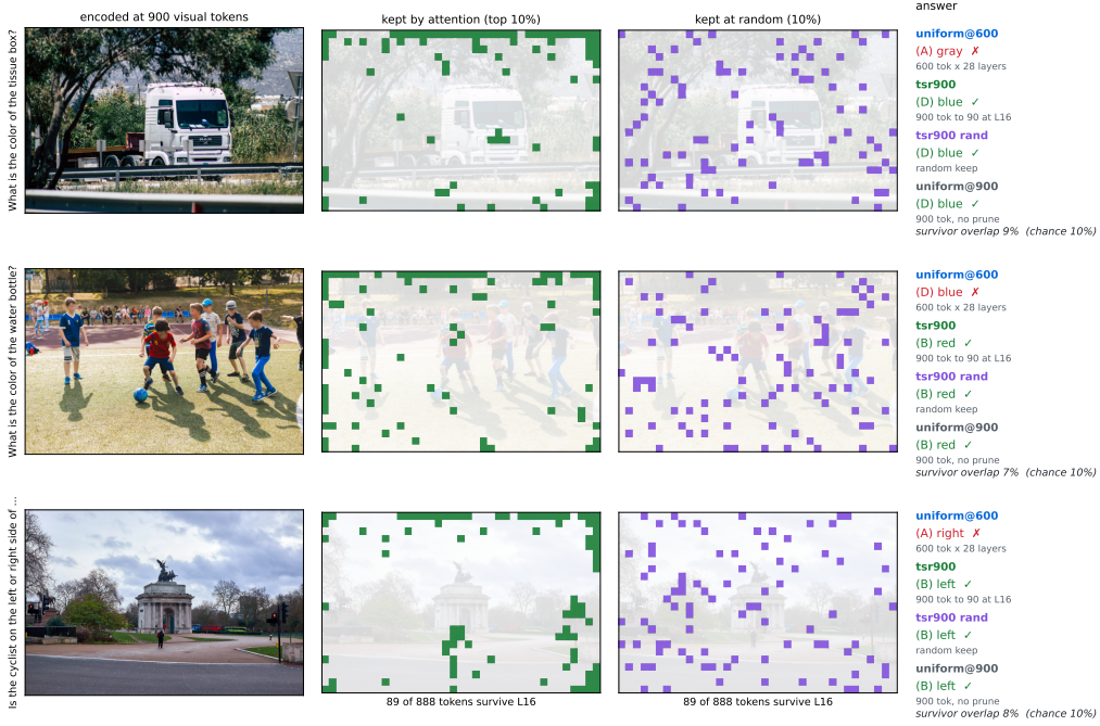
Figure 5: What survives the transport boundary, and why the choice of survivor does not matter (Qwen3-VL-2B). Of 888 visual tokens, 89 are carried past L16. Ranking them by attention selects mostly border tokens — the same sink Figure 4 exposes — while a random keep of the same size overlaps it by only 7–9%, at the 10% chance rate. Both give the same answer, and so does not pruning at all, on all three items; across the benchmark attention-keep and random-keep agree on 96.3% of items (70.2% vs 68.6% accuracy). The gain over the bar is resolution, not selection. Selection rule for the examples: TSR correct, the equal-compute bar wrong, and random keep agreeing with attention keep; 15 items qualify.
