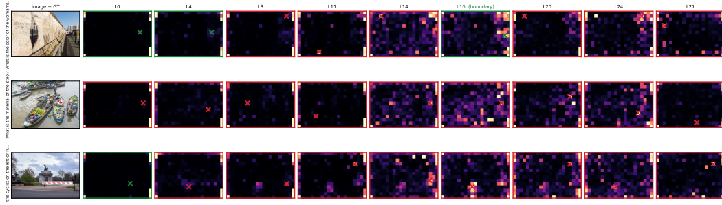
Figure 10: The same image, the same question, a different answer about where to look at every depth. Each panel is one layer’s attention over image cells (colour clipped at the 98th percentile so the serialisation sink does not wash out the structure); the cross is that layer’s ring-masked arg-max, green where the resulting crop would cover the evidence and red where it would not. Nothing about the input changes across a row. Only the read-out depth does.
