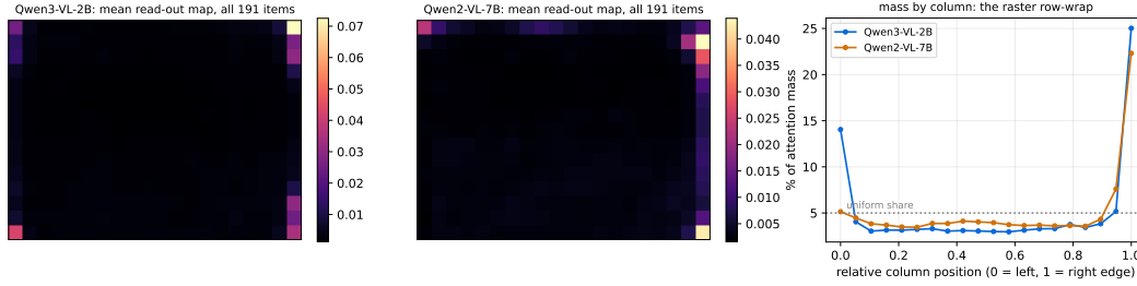
Figure 16: The serialisation sink, averaged over the benchmark. Each item’s read-out map is resampled to a common grid and averaged over all 191 items. Mass concentrates in the last column — the token before a raster row-wrap — on both checkpoints, at roughly four times the uniform share. This is what the outer-ring mask in every deployed implementation is patching around.
