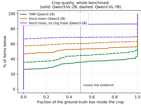
Figure 17: Crop quality over the whole benchmark. Cumulative distribution of the fraction of the ground-truth box captured by the crop. Without the ring mask the block-mean rule is close to useless; with it, it is usable; TWR is better than both and barely uses the mask.
