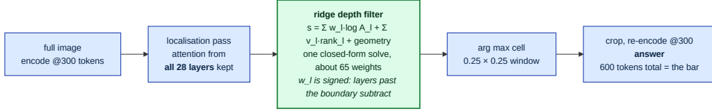
Figure 2: Policy I: Transport-Weighted Read-out (TWR). One localisation pass, every layer’s attention kept, a single closed-form solve that re-weights depths, and a crop. All 28 layers enter the score. The fitted weights are signed, but sign is not the mechanism: a non-negative refit retains the whole advantage while zeroing 44 of 56 per-layer coefficients (§K).
