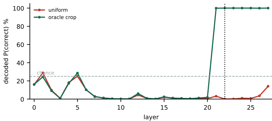
Qwen3-VL-2B (correct option: C)
