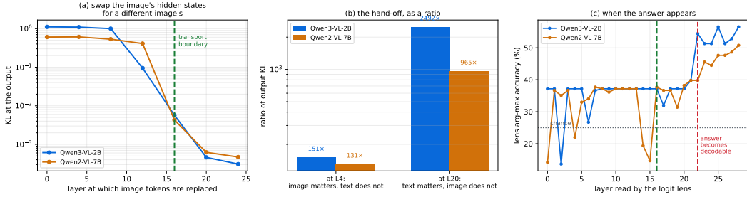
Figure 17: (a) Replacing the image tokens’ hidden states at layer \ell with a different image’s: the output effect falls three orders of magnitude across the boundary. (b) The hand-off as a ratio: early, the image dominates and the text is inert; late, exactly the reverse. (c) Logit lens at the answer position: the correct option becomes decodable only in the last quarter of the stack.
