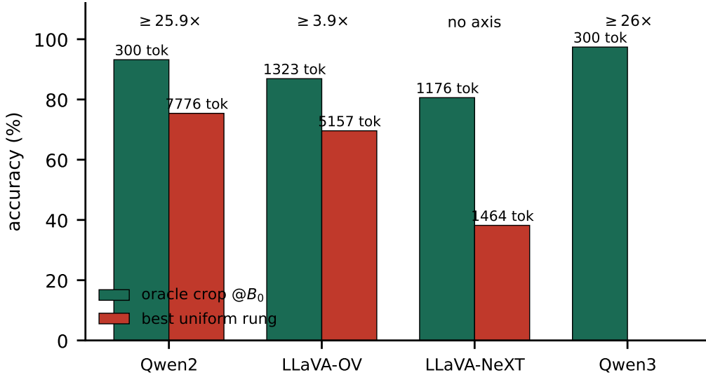
Figure 13: Allocation vs budget. Oracle crop at the base budget (green) against the best uniform rung each model reaches (red; token counts annotated). The exchange rate is the ratio of the token counts at which the two arms score what they score; no uniform rung matches the crop, so each rate is a lower bound.
