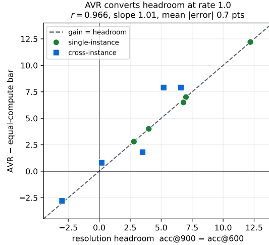
Figure 14: AVR is a resolution converter. Its gain over the equal-compute bar tracks the headroom the checkpoint already has, at rate 1.0. The one cell where AVR loses is the one cell where the baseline itself is worse at 900 tokens than at 600.
