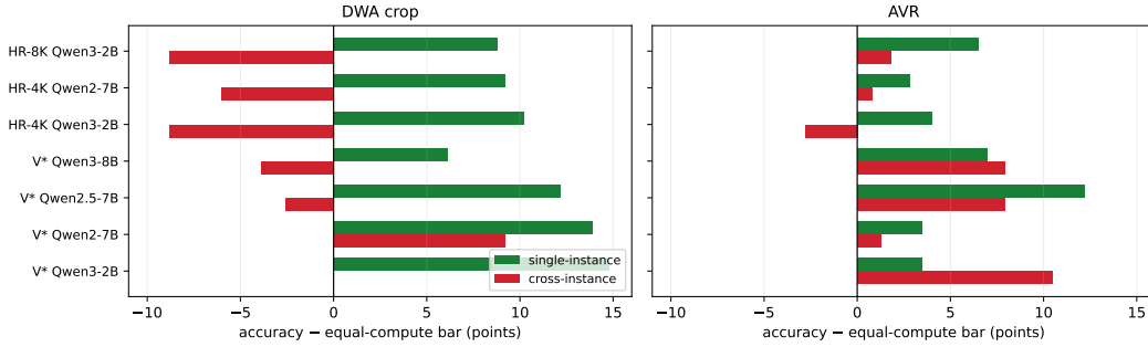
Figure 15: The scope law. Cropping is worth +6 to +15 points on single-instance questions in all seven cells and is negative on cross-instance in six of them. AVR is positive on both strata in six of seven, and gives up most of the single-instance gain to get there. The two policies are not variants of one method.
