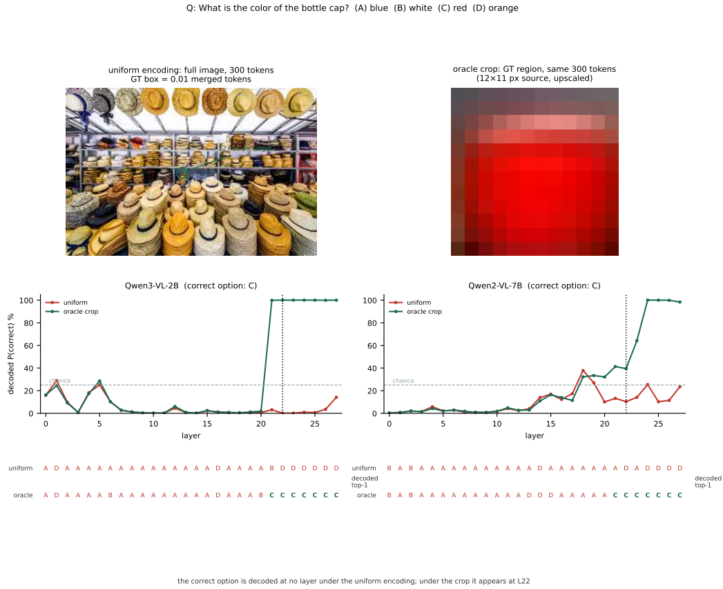
Figure 11: The lens on a real item. V*Bench direct_attributes/96: “What is the color of the bottle cap?” (A) blue (B) white (C) red (D) orange. The target is a 12 \times 11 px region, 0.01 merged tokens at the 300-token pass. Top: the image as the uniform pass sees it (target circled) and the oracle crop. Middle: the decoded probability of the correct option per layer. Bottom: the decoded top-1 option letter at every layer, both arms. Under the uniform encoding the correct option is decoded at no layer; after the crop it appears at L22 and stays.
