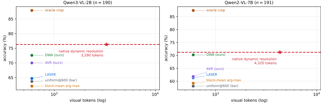
Figure 16: Accuracy against visual-token compute, V*Bench. The dashed line is the model run at its own native dynamic resolution. Our two policies sit on it at 14–18% of its compute; the published rules sit significantly below it; and a perfectly placed 600-token crop sits well above it. Placement is worth more than 5–7 \times the tokens.
