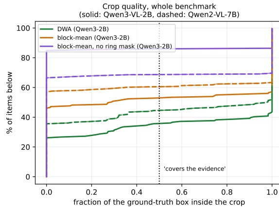
Figure 27: Crop quality over the whole benchmark. Cumulative distribution of the fraction of the ground-truth box captured by the crop. Without the ring mask the block-mean rule is close to useless; with it, it is usable; DWA is better than both and barely uses the mask.
