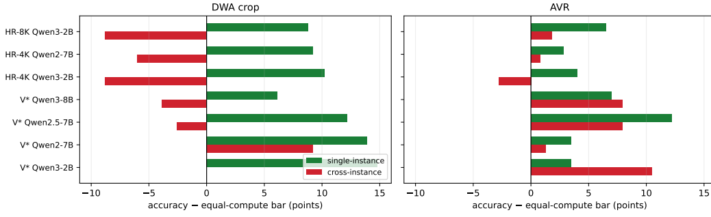
Figure 18: The scope law. Cropping is worth +6 to +15 points on single-instance questions in all seven cells and is negative on cross-instance in six of them. AVR is positive on both strata in six of seven, and gives up most of the single-instance gain to get there. The two policies are not variants of one method.
