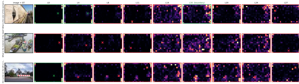
Figure 20: The same image, the same question, a different answer about where to look at every depth. Each panel is one layer’s attention over image cells (colour clipped at the 98th percentile so the serialisation sink does not wash out the structure); the cross is that layer’s ring-masked arg-max, green where the resulting crop would cover the evidence and red where it would not. Nothing about the input changes across a row. Only the read-out depth does.
