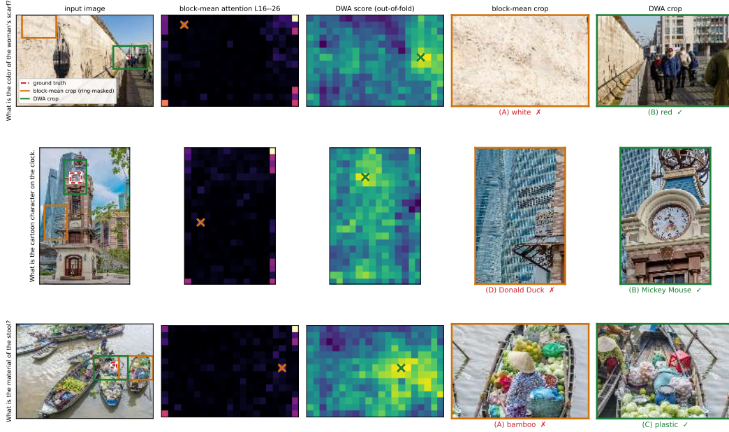
Figure 6: Crop placement and answer changes on Qwen3-VL-2B. The panels show the full image, block-mean attention, held-out DWA scores, and the two resulting crops. Both rules exclude the outer grid ring. These are the first three question IDs among nine qualifying single-instance examples where DWA covers at least half of the evidence box and answers correctly, the block mean does neither, and the recomputed DWA location matches the recorded run. They illustrate successful corrections under this selection criterion.
