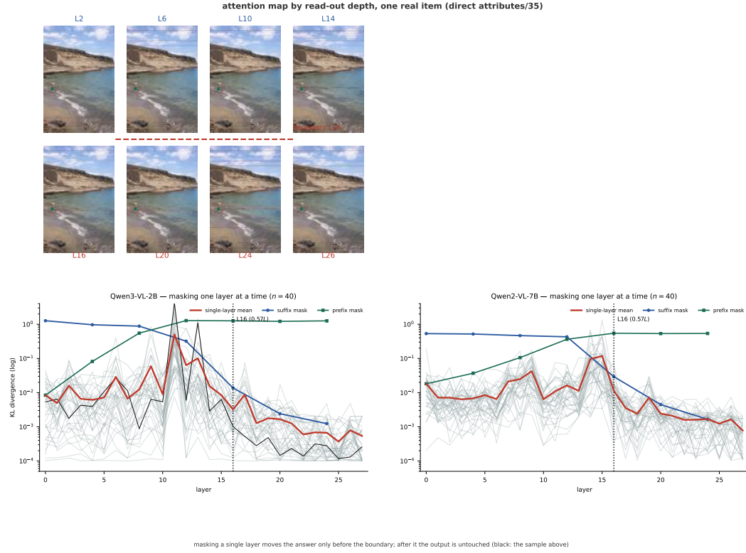
Figure 5: The boundary on real items. Top: one V*Bench item’s attention map at selected read-out depths, pre-boundary above and post-boundary below the dashed line; the late maps collapse onto a row-boundary band. Bottom: single-layer masking KL for all 40 calibrated items (thin), the mean (bold), and the prefix/suffix schedules, both models, with the boundary at L16 (0.57L). Black: the sample shown above.
