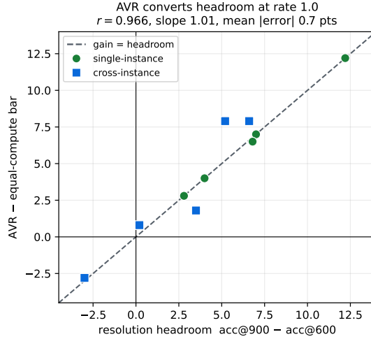
Figure 17: AVR is a resolution converter. Its gain over the equal-compute bar tracks the headroom the checkpoint already has, at rate 1.0. The one cell where AVR loses is the one cell where the baseline itself is worse at 900 tokens than at 600.
