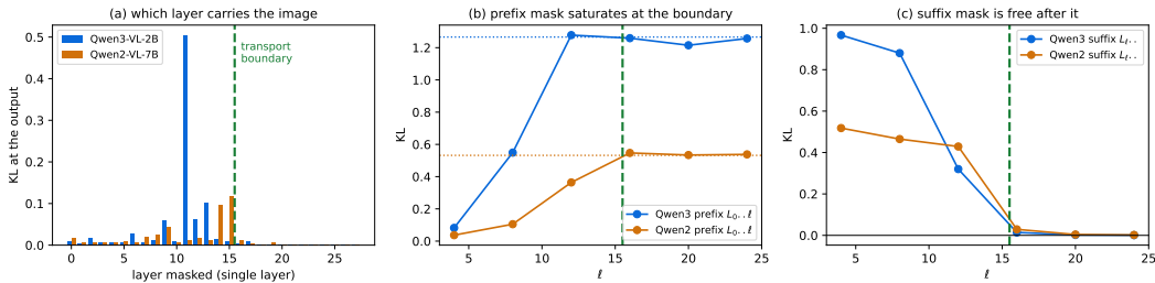
Figure 9: The transport measurement. (a) Masking one layer’s image attention at a time: the effect is concentrated well before the boundary and is at or below 0.0023 from L20 on both models. (b) Masking a prefix L_{0..l} reaches the full-mask value (dotted) once l passes the window. (c) Masking a suffix L_{l..end} costs nothing once l is past it. Three readings, one boundary.
