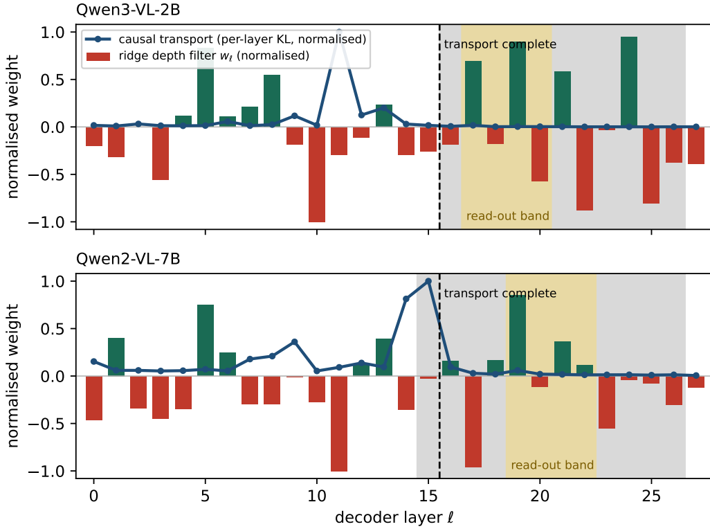
Figure 4: Fitted depth weights and output sensitivity. Normalised DWA log-attention coefficients and normalised single-layer masking KL for the two core checkpoints. The marked boundary indicates an approximate transition in output sensitivity. The bars show fitted log-attention coefficients; rank and spatial coefficients are omitted.
