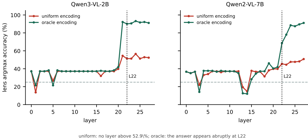
Figure 13: The answer is not in the stack. Per-layer logit-lens accuracy under the uniform encoding (red) and the oracle crop (green), both models. Uniform: flat, no layer above 52.9% and none holding an answer that is later lost. Oracle: the answer becomes decodable abruptly at L22, taking most of the gain in one transition; the Qwen2 step is one layer later.
