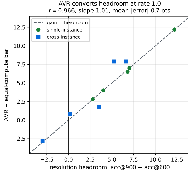
Figure 8: AVR gain and the benefit of higher input resolution. Each point is one of ten reported benchmark-checkpoint-stratum combinations with an unmodified 900-token reference. The horizontal axis measures its accuracy gain over 600 tokens; the vertical axis measures AVR’s gain over that same reference budget. The diagonal indicates equal gains. Both axes share the same 600-token reference.
