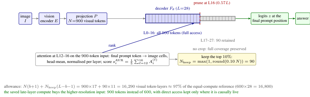
Figure 3: AVR: prune at the boundary, spend the saving on resolution. The image is encoded at 900 tokens (instead of the reference’s 600) and every layer keeps full visual access through L16. The final prompt token’s attention over layers 12–16 ranks the tokens; the top 10% ( N_{\text{keep}}=90 ) are retained, and from L17 onward only those keys remain accessible. The allowance N(b+1) + N_{\text{keep}}(L-b-1) = 900 \times 17 + 90 \times 11 = 16,290 visual token-layers is \approx 97\% of the equal-compute reference ( 600 \times 28 = 16,800 ). No crop is applied: full coverage is preserved.
