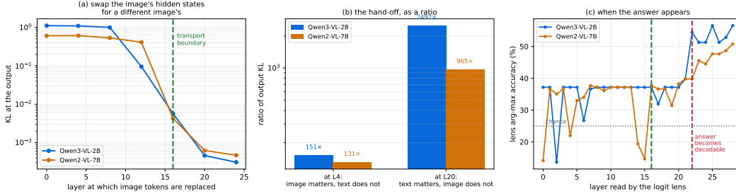
Figure 10: (a) Replacing the image tokens’ hidden states at layer \ell with a different image’s: the output effect falls three orders of magnitude across the boundary. (b) The hand-off as a ratio: early, the image dominates and the text is inert; late, exactly the reverse. (c) Logit lens at the answer position: the correct option becomes decodable only in the last quarter of the stack.
