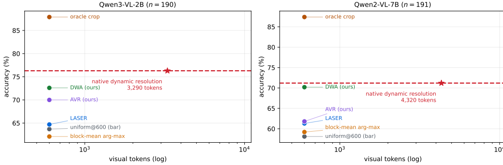
Figure 19: Accuracy against visual-token compute, V*Bench. The dashed line is the model run at its own native dynamic resolution. Our two policies sit on it at 14–18% of its compute; the published rules sit significantly below it; and a perfectly placed 600-token crop sits well above it. Placement is worth more than 5–7 \times the tokens.
