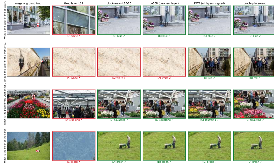
Figure 22: Five placement rules, same items, same budget. Selection rule: single-instance items on which the oracle crop is correct, so the ceiling behaves like a ceiling, and on which DWA is correct while the fixed-layer rule is not; 61 items qualify and the first four by question id are shown. The fixed mid-layer recipe crops glass, masonry and sky.
