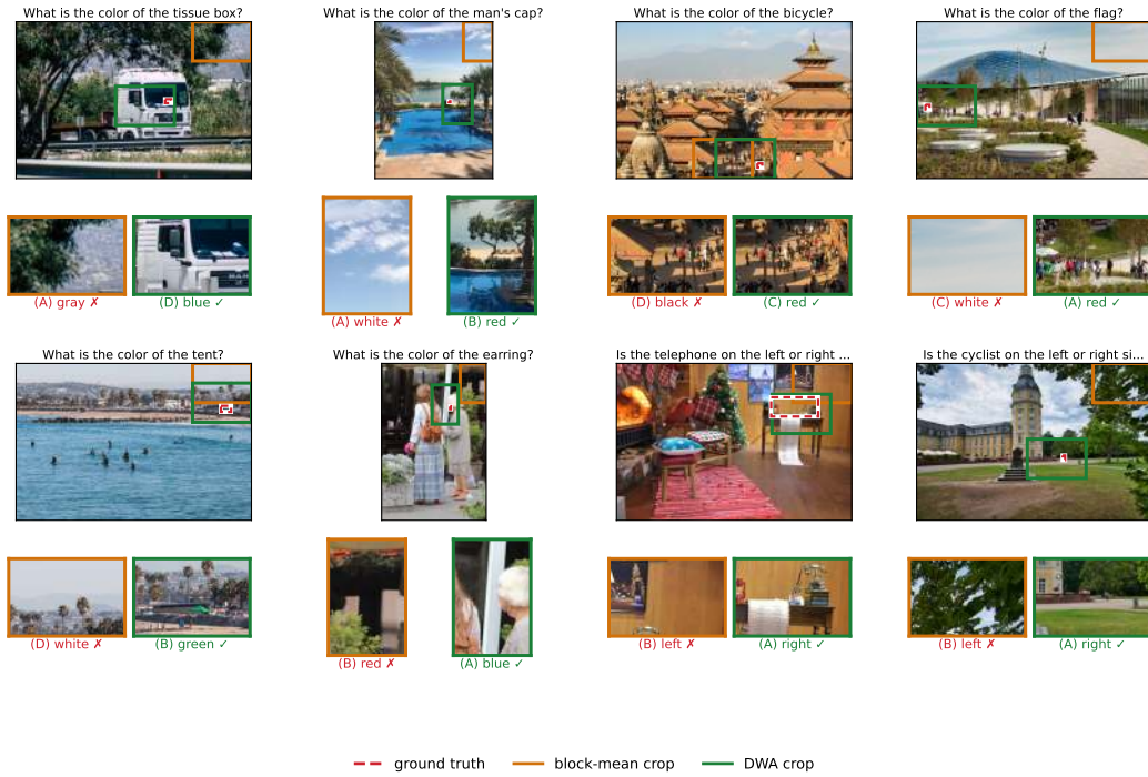
Figure 24: The same eight-item view on Qwen2-VL-7B. The failure mode is the same on a different model family and a different parameter count.
