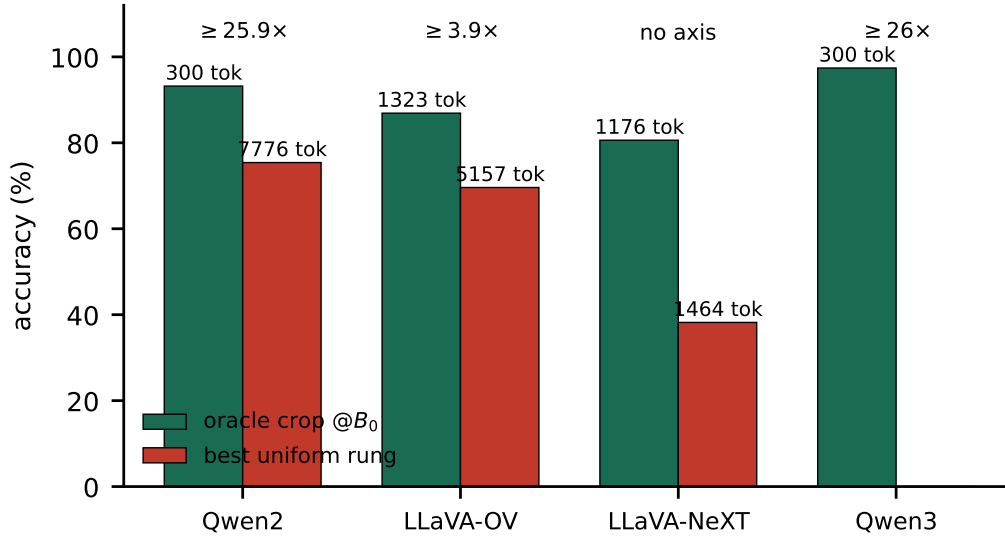
Figure 16: Allocation vs budget. Oracle crop at the base budget (green) against the best uniform rung each model reaches (red; token counts annotated). The exchange rate is the ratio of the token counts at which the two arms score what they score; no uniform rung matches the crop, so each rate is a lower bound.
