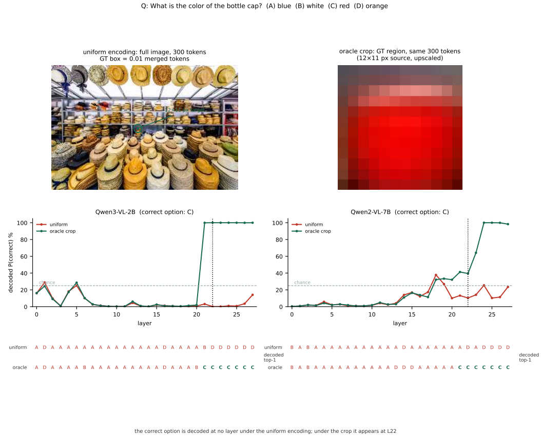
Figure 14: The lens on a real item. V*Bench direct_attributes/96: “What is the color of the bottle cap?” (A) blue (B) white (C) red (D) orange. The target is a 12 \times 11 px region, 0.01 merged tokens at the 300-token pass. Top: the image as the uniform pass sees it (target circled) and the oracle crop. Middle: the decoded probability of the correct option per layer. Bottom: the decoded top-1 option letter at every layer, both arms. Under the uniform encoding the correct option is decoded at no layer; after the crop it appears at L22 and stays.
