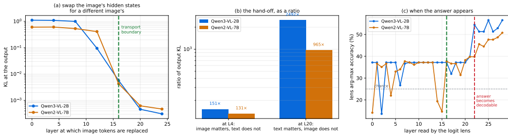
Figure 7: (a) Replacing the image tokens’ hidden states at layer l with a different image’s: the output effect falls three orders of magnitude across the boundary. (b) The hand-off as a ratio: early, the image dominates and the text is inert; late, exactly the reverse. (c) Logit lens at the answer position: the correct option becomes decodable only in the last quarter of the stack.
