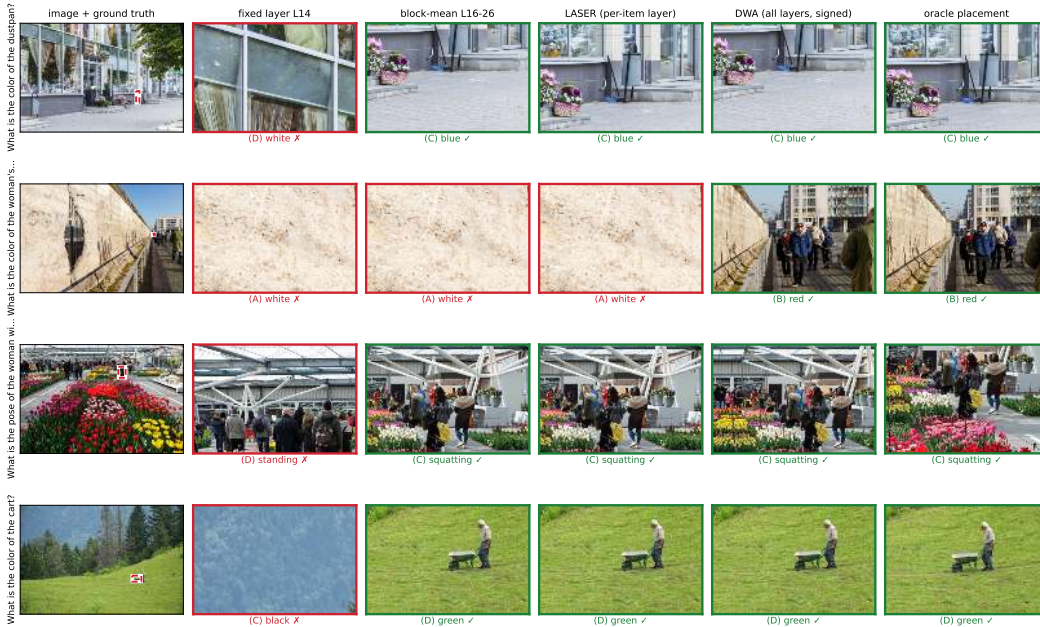
Figure 14: Five placement rules, same items, same budget. Selection rule: single-instance items on which the oracle crop is correct, so the ceiling behaves like a ceiling, and on which DWA is correct while the fixed-layer rule is not; 61 items qualify and the first four by question id are shown. The fixed mid-layer recipe crops glass, masonry and sky.
