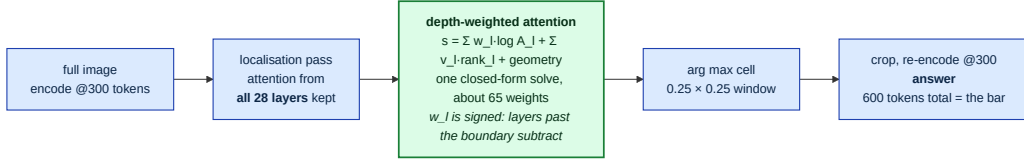
Figure 3: Policy I: Depth-Weighted Attention (DWA) . One localisation pass, every layer’s attention kept, a single closed-form solve that re-weights depths, and a crop. All 28 layers enter the score. The fitted weights are signed, but sign is not the mechanism: a non-negative refit retains the whole advantage while zeroing 44 of 56 per-layer coefficients (§M).
