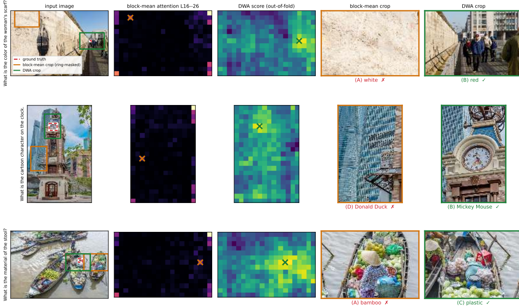
Figure 5: What the two read-out rules see, on real V*Bench items (Qwen3-VL-2B). The block-mean arg-max is shown as the paper evaluates it, which masks the grid’s outer ring before taking the arg-max — and that mask is doing very unequal amounts of work. Without it, the block-mean arg-max lands in the grid’s last column , the position before a raster row-wrap, on 84.8% and 61.8% of items across the two checkpoints against a 5.0% chance rate, and covers half the ground-truth box on only 13.6% of items; the ring mask lifts that to 46.6% and 39.3% across the two checkpoints. DWA covers 63.9% and 55.0%, and barely uses the mask: it is worth +0.012 and +0.003 mean coverage to DWA against +0.336 and +0.079 to block-mean, an order of magnitude on both. DWA removes the serialisation sink by a supervised depth weighting that suppresses the item-independent component, not by patching the geometry and not by the signs of the fitted weights (Appendix M). Examples are not hand-picked: we take single-instance items where the DWA crop covers the box and the block-mean crop does not and the answers flip accordingly, restricted to items where the recomputed out-of-fold DWA cell reproduces the logged run exactly. Nine items qualify; these are the first three by question id.
