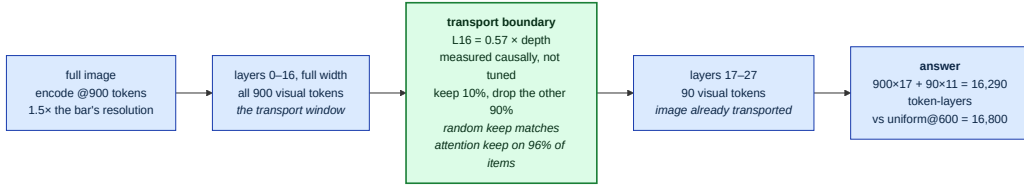
Figure 4: Policy II, adaptive visual resolution. Spend the compute the inert late-layer visual tokens would have used on resolution inside the window where the image is actually read. The prune depth is read off the causal measurement rather than tuned, and nothing spatial is discarded before the boundary.
