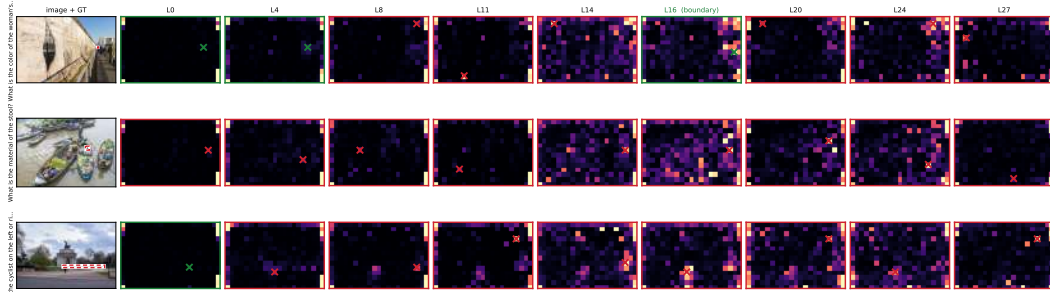
Figure 12: The same image, the same question, a different answer about where to look at every depth. Each panel is one layer’s attention over image cells (colour clipped at the 98th percentile so the serialisation sink does not wash out the structure); the cross is that layer’s ring-masked arg-max, green where the resulting crop would cover the evidence and red where it would not. Nothing about the input changes across a row. Only the read-out depth does.
