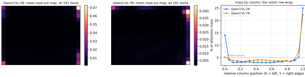
Figure 18: The serialisation sink, averaged over the benchmark. Each item’s read-out map is resampled to a common grid and averaged over all 191 items. Mass concentrates in the last column — the token before a raster row-wrap — on both checkpoints, at roughly four times the uniform share. This is what the outer-ring mask in every deployed implementation is patching around.
