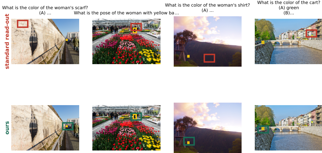
Figure 5: Items where the standard read-out misses and a learned one succeeds. Yellow: queried object. Red/green: the crop each read-out selects.
