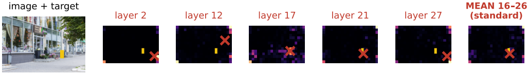
Figure 1: The layers disagree, and the standard read-out averages the disagreement away. One V*Bench item; the yellow box is the queried object. Each panel is attention over image positions at one layer; \times marks its maximum (green inside the target, red outside). Individual layers disagree sharply. The rightmost panel is the read-out used in practice — the mean over layers 16–26 — whose maximum lands outside the target.
