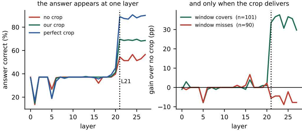
Figure 4: Cropping restores an answer-formation step; it does not improve reasoning. Left: the answer read out at every layer. Right: the same gain split by whether the crop contained the evidence.
