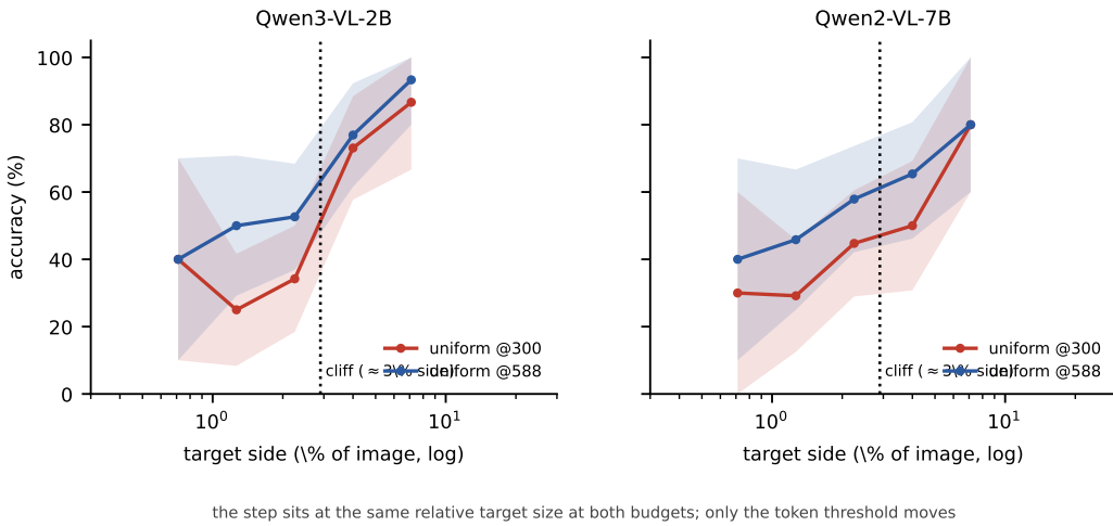
Figure 10: The cliff does not move with budget. Accuracy vs the target’s side as a fraction of the image, at 300 and 588 tokens, both models. The step sits at the same relative size ( \approx 3\% of the side) at both budgets: doubling the uniform budget moves the token threshold but not the cliff.
