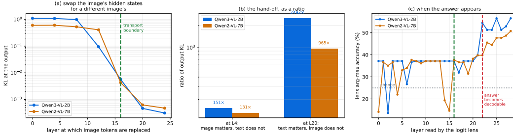
Figure 8: (a) Replacing the image tokens’ hidden states at layer \ell with a different image’s: the output effect falls three orders of magnitude across the boundary. (b) The hand-off as a ratio: early, the image dominates and the text is inert; late, exactly the reverse. (c) Logit lens at the answer position: the correct option becomes decodable only in the last quarter of the stack.
