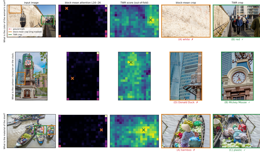
Figure 4: What the two read-out rules see, on real V*Bench items (Qwen3-VL-2B). The block-mean arg-max is shown as the paper evaluates it, which masks the grid’s outer ring before taking the arg-max — and that mask is doing very unequal amounts of work. Without it, the block-mean arg-max lands in the grid’s last column , the position before a raster row-wrap, on 84.8% and 61.8% of items across the two checkpoints against a 5.0% chance rate, and covers half the ground-truth box on only 13.6% of items; the ring mask lifts that to 46.6% and 39.3% across the two checkpoints. TWR covers 63.9% and 55.0%, and barely uses the mask: it is worth +0.012 and +0.003 mean coverage to TWR against +0.336 and +0.079 to block-mean, an order of magnitude on both. TWR removes the serialisation sink by giving the post-boundary layers negative weight rather than by patching the geometry. Examples are not hand-picked : we take single-instance items where the TWR crop covers the box and the block-mean crop does not and the answers flip accordingly, restricted to items where the recomputed out-of-fold TWR cell reproduces the logged run exactly. Nine items qualify; these are the first three by question id.
