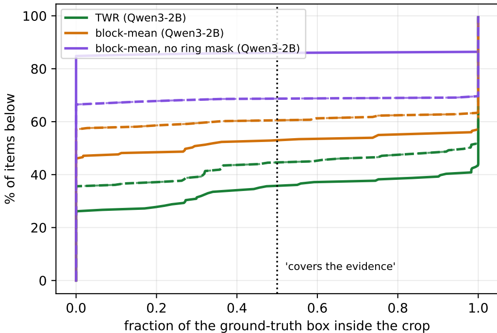
Crop quality, whole benchmark (solid: Qwen3-VL-2B, dashed: Qwen2-VL-7B)
