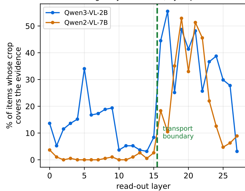
single-layer read-out, by depth
