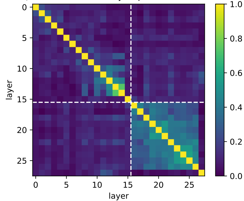
Qwen3-VL-2B: do two layers pick the same cell?
