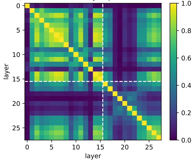
Qwen2-VL-7B: do two layers pick the same cell?
