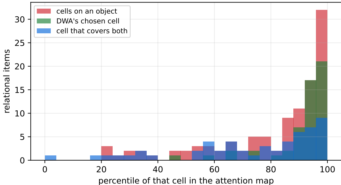
What the read-out ranks highly, and what it needs
