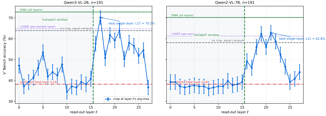
Figure 5: Accuracy when only the crop read-out layer changes. The layer sweep uses 191 V*Bench examples per checkpoint; error bars show one standard error. The fixed-layer and LASER (Zhu et al., 2026) lines denote the placement controls defined in Sec. 4. The dashed boundary is the approximate transition identified by masking.
