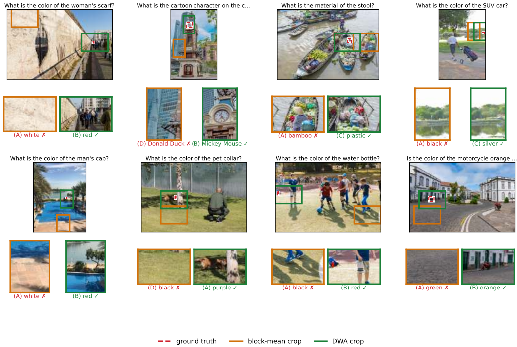
Figure 21: Eight inferences, Qwen3-VL-2B. Top of each cell: the image with the ground-truth box, the block-mean crop and the DWA crop. Below: the two crops the model actually answers from, with its answer.
