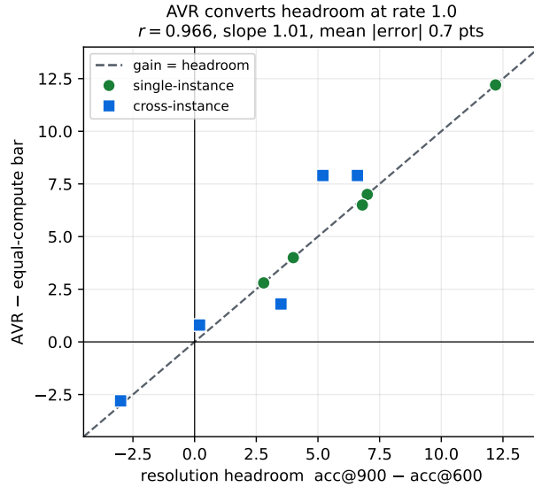
Figure 6: AVR gain and the benefit of higher input resolution. Each point is one of ten reported benchmark-checkpoint-stratum combinations with an unmodified 900-token reference. The horizontal axis measures its accuracy gain over 600 tokens; the vertical axis measures AVR’s gain over that same reference budget. The diagonal indicates equal gains. Both axes share the same 600-token reference.
