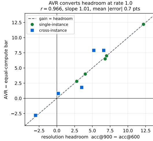
Figure 15: AVR is a resolution converter. Its gain over the equal-compute bar tracks the headroom the checkpoint already has, at rate 1.0. The one cell where AVR loses is the one cell where the baseline itself is worse at 900 tokens than at 600.
