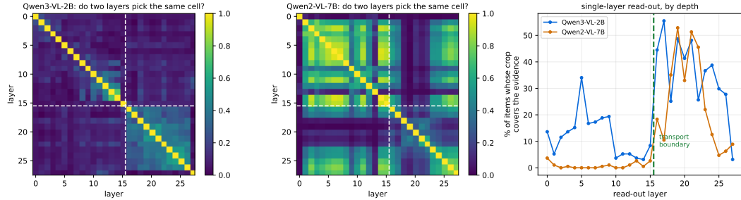
Figure 19: Left, centre: two layers rarely choose the same cell. Mean off-diagonal agreement is 13.8% and 38.1%; the block structure splits at the transport boundary (dashed). Right: and only the layers after the boundary are worth reading. The fraction of items whose single-layer crop covers the evidence is at or below 20% everywhere before the boundary, jumps immediately after it, and decays again toward the output. This is the paper’s central claim in one curve: the usable placement signal exists only after transport has finished.
