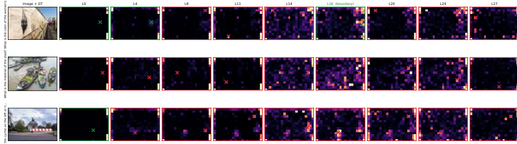
Figure 18: The same image, the same question, a different answer about where to look at every depth. Each panel is one layer’s attention over image cells (colour clipped at the 98th percentile so the serialisation sink does not wash out the structure); the cross is that layer’s ring-masked arg-max, green where the resulting crop would cover the evidence and red where it would not. Nothing about the input changes across a row. Only the read-out depth does.
