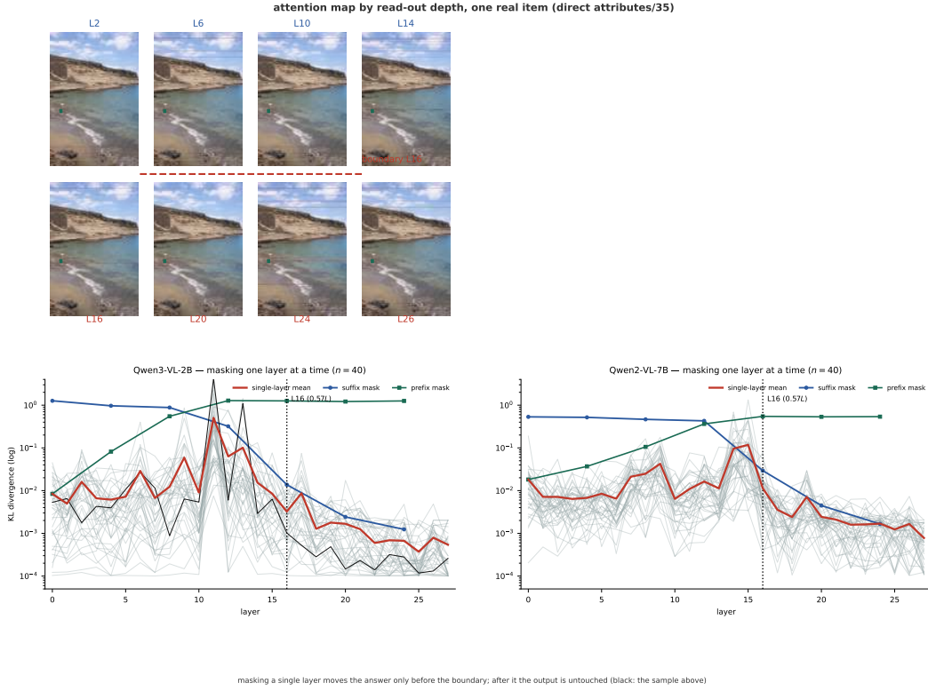
Figure 3: The boundary on real items. Top: one V*Bench item’s attention map at selected read-out depths, pre-boundary above and post-boundary below the dashed line; the late maps collapse onto a row-boundary band. Bottom: single-layer masking KL for all 40 calibrated items (thin), the mean (bold), and the prefix/suffix schedules, both models, with the boundary at L16 (0.57L). Black: the sample shown above.
