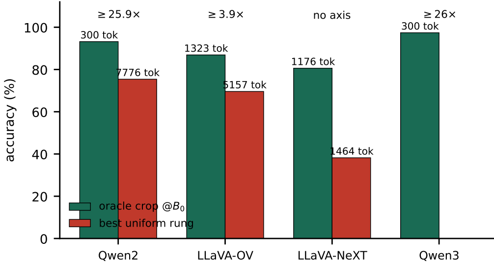
Figure 14: Allocation vs budget. Oracle crop at the base budget (green) against the best uniform rung each model reaches (red; token counts annotated). The exchange rate is the ratio of the token counts at which the two arms score what they score; no uniform rung matches the crop, so each rate is a lower bound.
