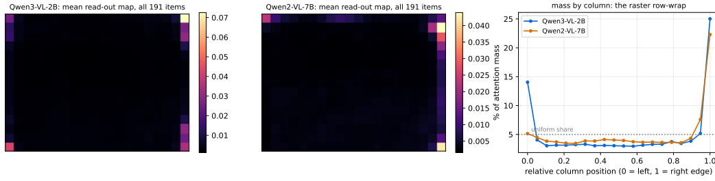
Figure 24: The serialisation sink, averaged over the benchmark. Each item’s read-out map is resampled to a common grid and averaged over all 191 items. Mass concentrates in the last column — the token before a raster row-wrap — on both checkpoints, at roughly four times the uniform share. This is what the outer-ring mask in every deployed implementation is patching around.
