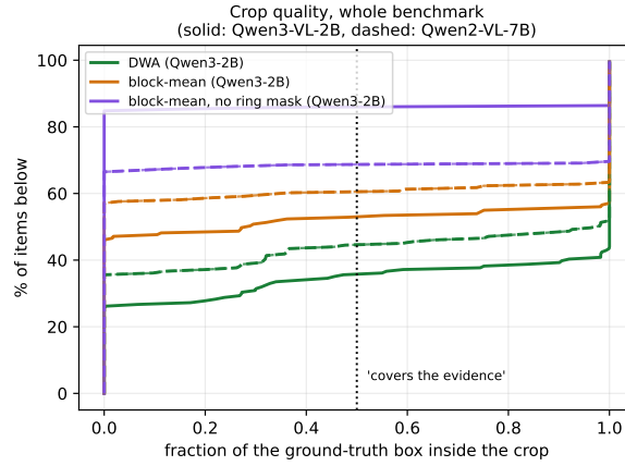
Figure 25: Crop quality over the whole benchmark. Cumulative distribution of the fraction of the ground-truth box captured by the crop. Without the ring mask the block-mean rule is close to useless; with it, it is usable; DWA is better than both and barely uses the mask.
