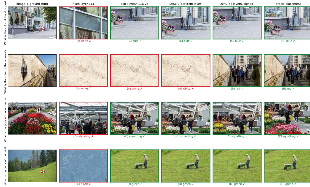
Figure 20: Five placement rules, same items, same budget. Selection rule: single-instance items on which the oracle crop is correct, so the ceiling behaves like a ceiling, and on which DWA is correct while the fixed-layer rule is not; 61 items qualify and the first four by question id are shown. The fixed mid-layer recipe crops glass, masonry and sky.
