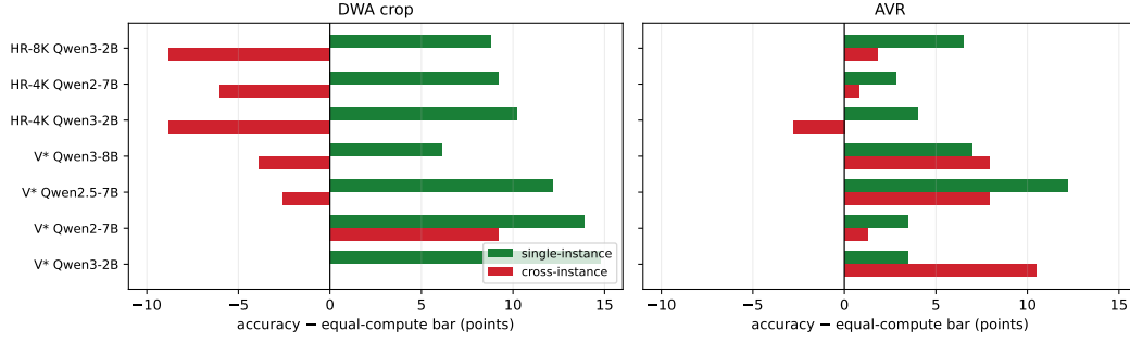
Figure 16: The scope law. Cropping is worth +6 to +15 points on single-instance questions in all seven cells and is negative on cross-instance in six of them. AVR is positive on both strata in six of seven, and gives up most of the single-instance gain to get there. The two policies are not variants of one method.
