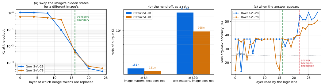
Figure 8: (a) Replacing the image tokens’ hidden states at layer l with a different image’s: the output effect falls three orders of magnitude across the boundary. (b) The hand-off as a ratio: early, the image dominates and the text is inert; late, exactly the reverse. (c) Logit lens at the answer position: the correct option becomes decodable only in the last quarter of the stack.
