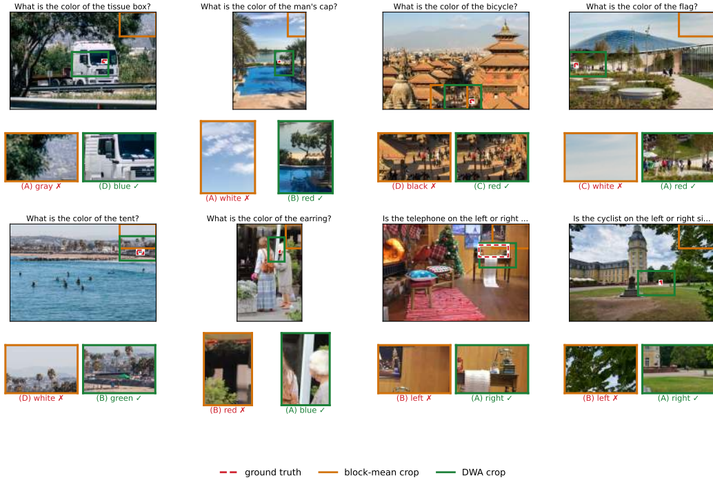
Figure 22: The same eight-item view on Qwen2-VL-7B. The failure mode is the same on a different model family and a different parameter count.
