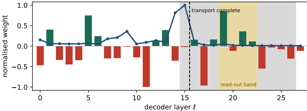
Qwen2-VL-7B
