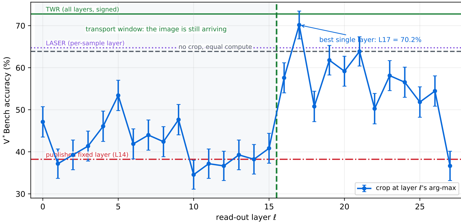
Where you read the attention map decides the method Qwen3-VL-2B, n=191 , every arm at \sim 600 visual tokens
