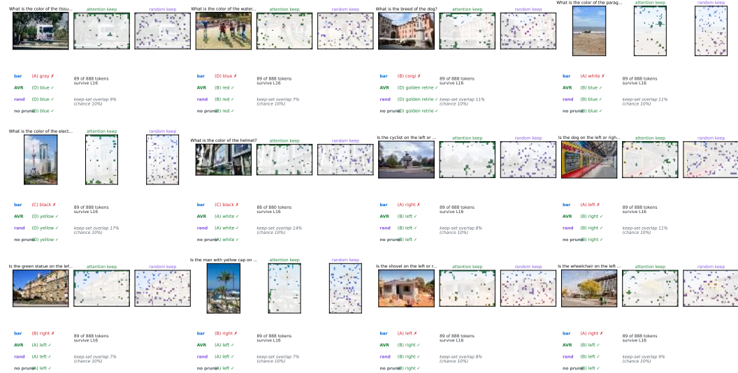
Figure 17: Twelve inferences under AVR. For each item: the image, the tokens kept by attention at the boundary, and an equally sized random keep. The two keep-sets overlap at close to the 10% chance rate and the model answers identically under both, and identically again without pruning at all.
