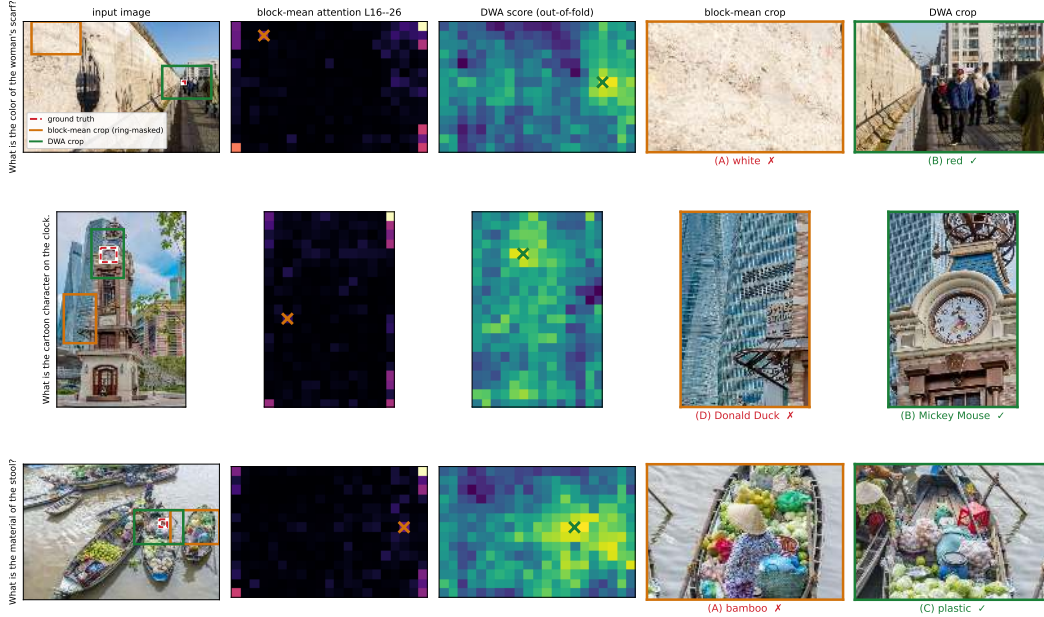
Figure 4: Crop placement and answer changes on Qwen3-VL-2B. The panels show the full image, block-mean attention, held-out DWA scores, and the two resulting crops. Both rules exclude the outer grid ring. These are the first three question IDs among nine qualifying single-instance examples where DWA covers at least half of the evidence box and answers correctly, the block mean does neither, and the recomputed DWA location matches the recorded run. They illustrate successful corrections under this selection criterion.
