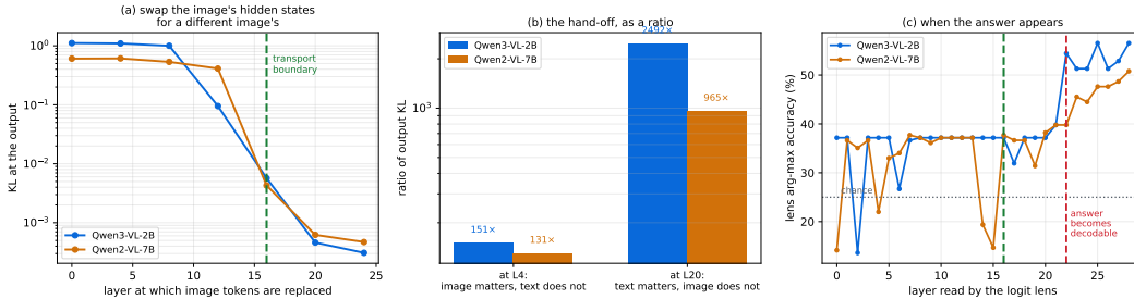
Figure 11: (a) Replacing the image tokens’ hidden states at layer \ell with a different image’s: the output effect falls three orders of magnitude across the boundary. (b) The hand-off as a ratio: early, the image dominates and the text is inert; late, exactly the reverse. (c) Logit lens at the answer position: the correct option becomes decodable only in the last quarter of the stack.
