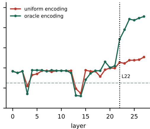
Qwen2-VL-7B
