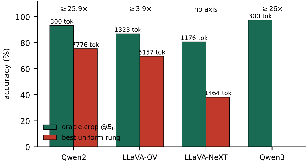
Figure 11: Allocation vs budget. Oracle crop at the base budget (green) against the best uniform rung each model reaches (red; token counts annotated). The exchange rate is the ratio of the token counts at which the two arms score what they score; no uniform rung matches the crop, so each rate is a lower bound.
