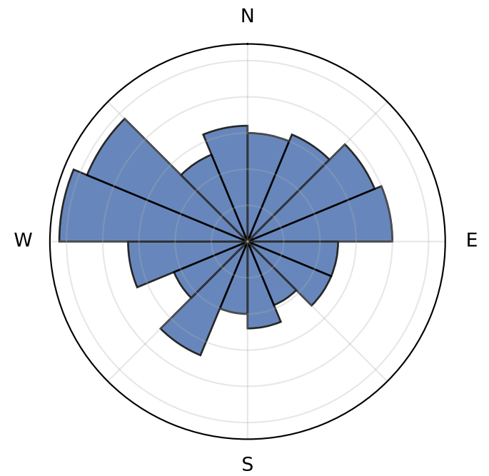
VLM Debate
