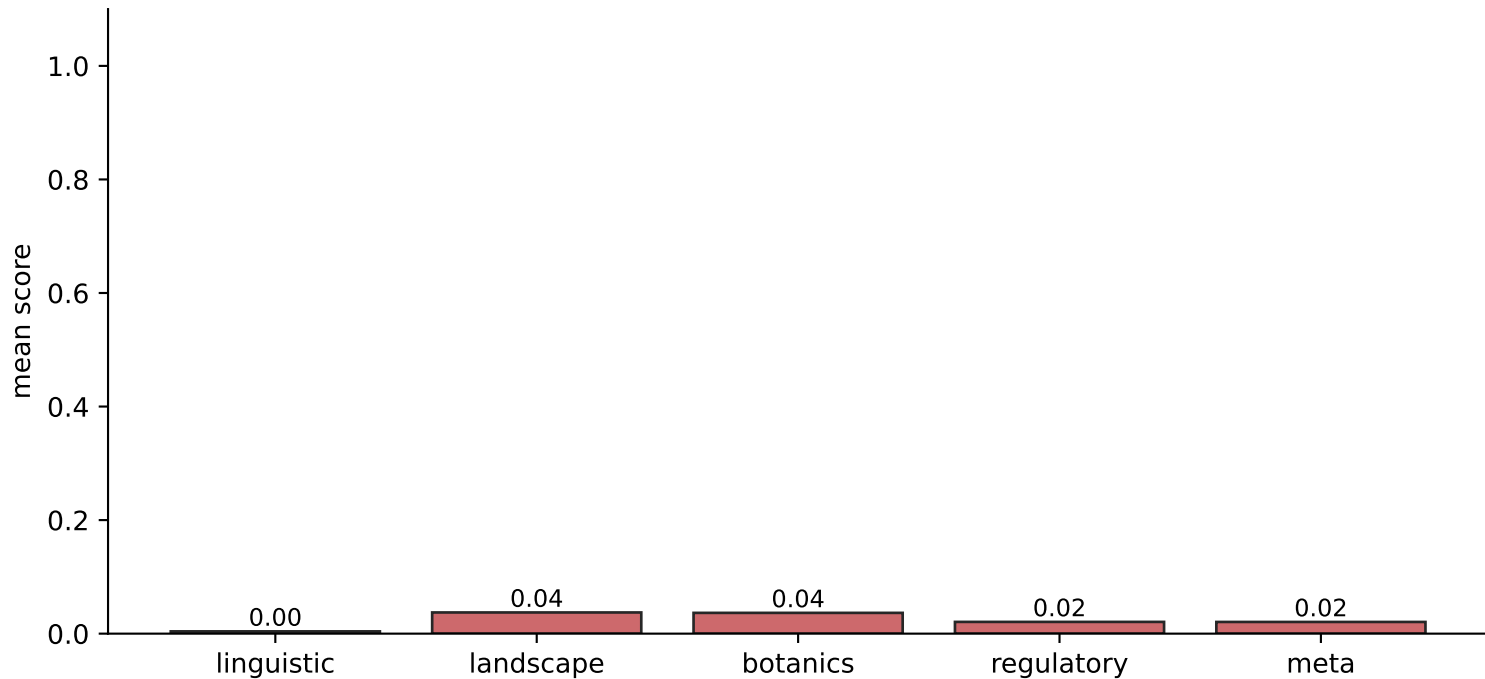
Per-agent hallucination score (0=clean, lower=better)
