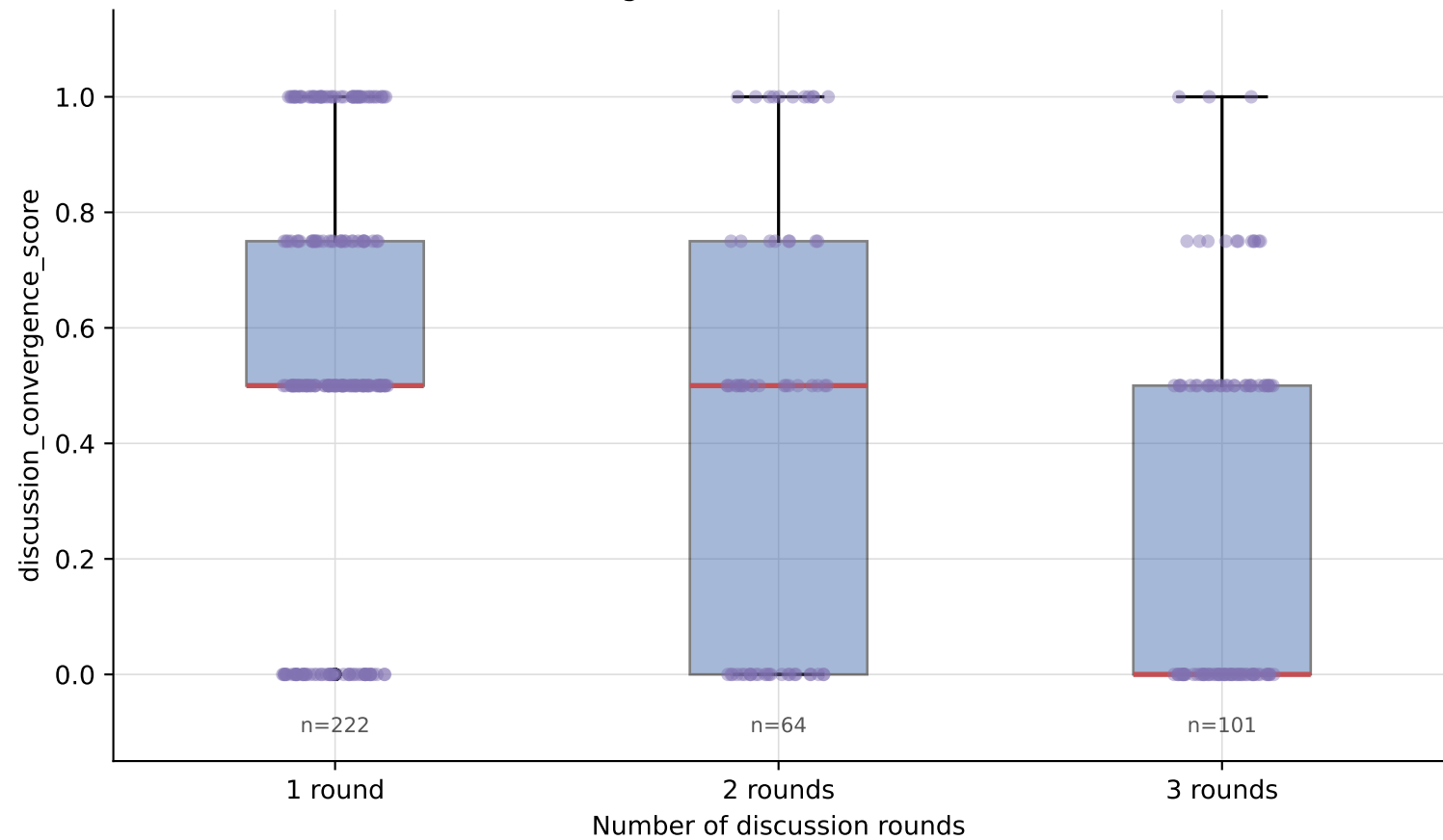
Discussion convergence score vs. number of hub rounds
