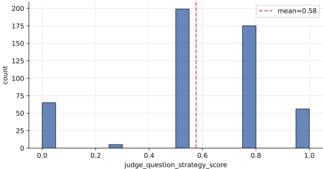
Judge question strategy score distribution per image
