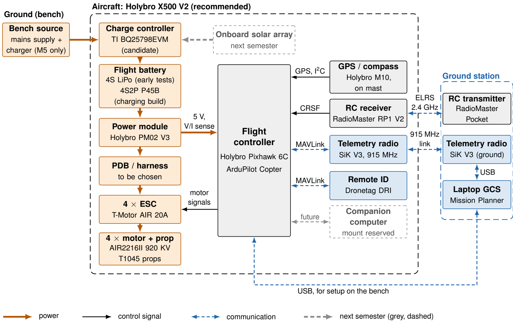
Figure 1. Thick arrows carry power, thin arrows carry control signals, and blue dashed arrows carry communication. The companion computer and the solar array are placeholders for next semester.
