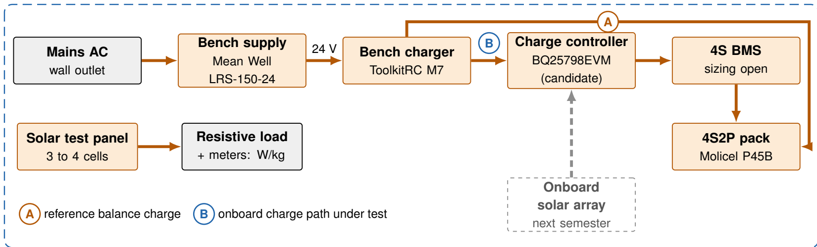
Figure 3. Electrical power paths. Grey dashed arrows and boxes are next-semester items.
