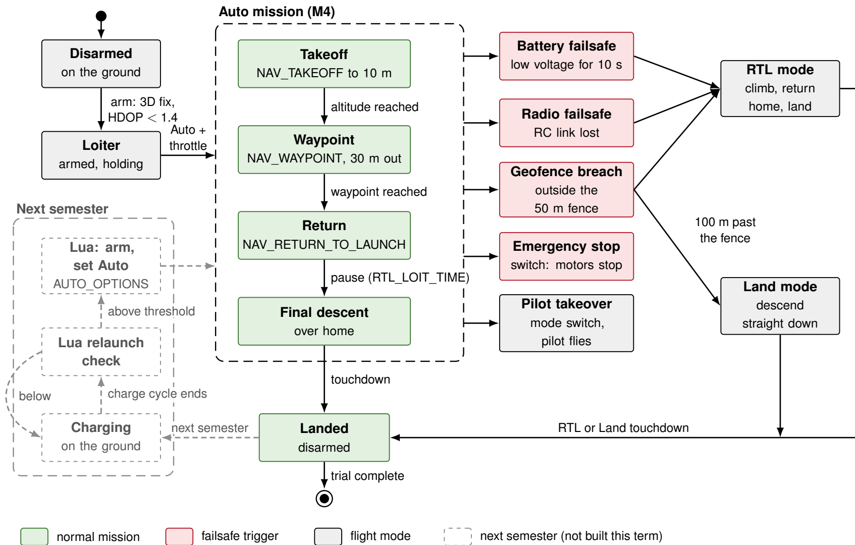
Figure 2. Mission and fault state machine. Everything outside the Next semester block is this semester's scope. The charge and relaunch states are next-semester work.
