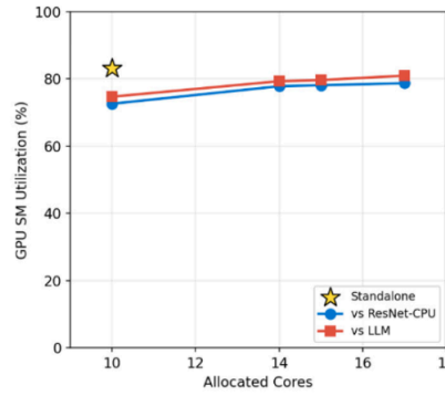
(b) ResNet-GPU
