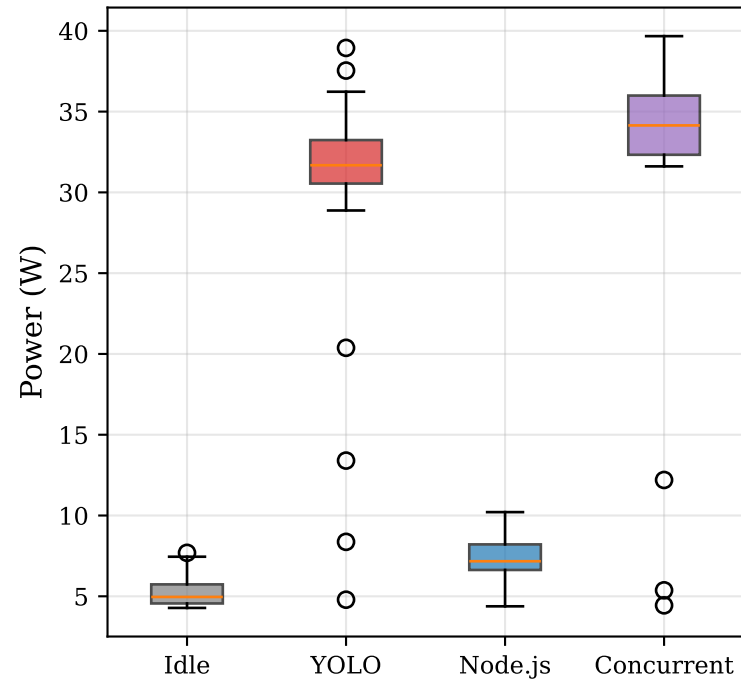
(A) CPU Power Distribution
