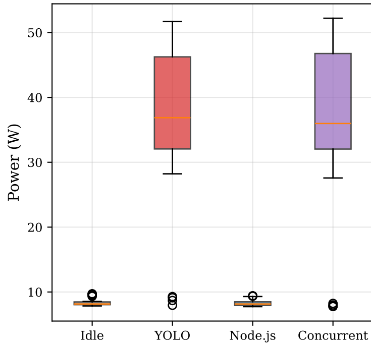
(B) GPU Power Distribution
