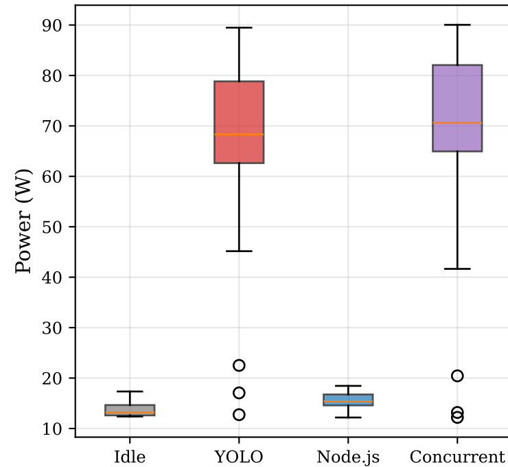
(C) Total Power Distribution
