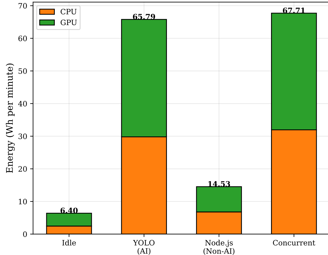
(A) Energy Consumption by Component
