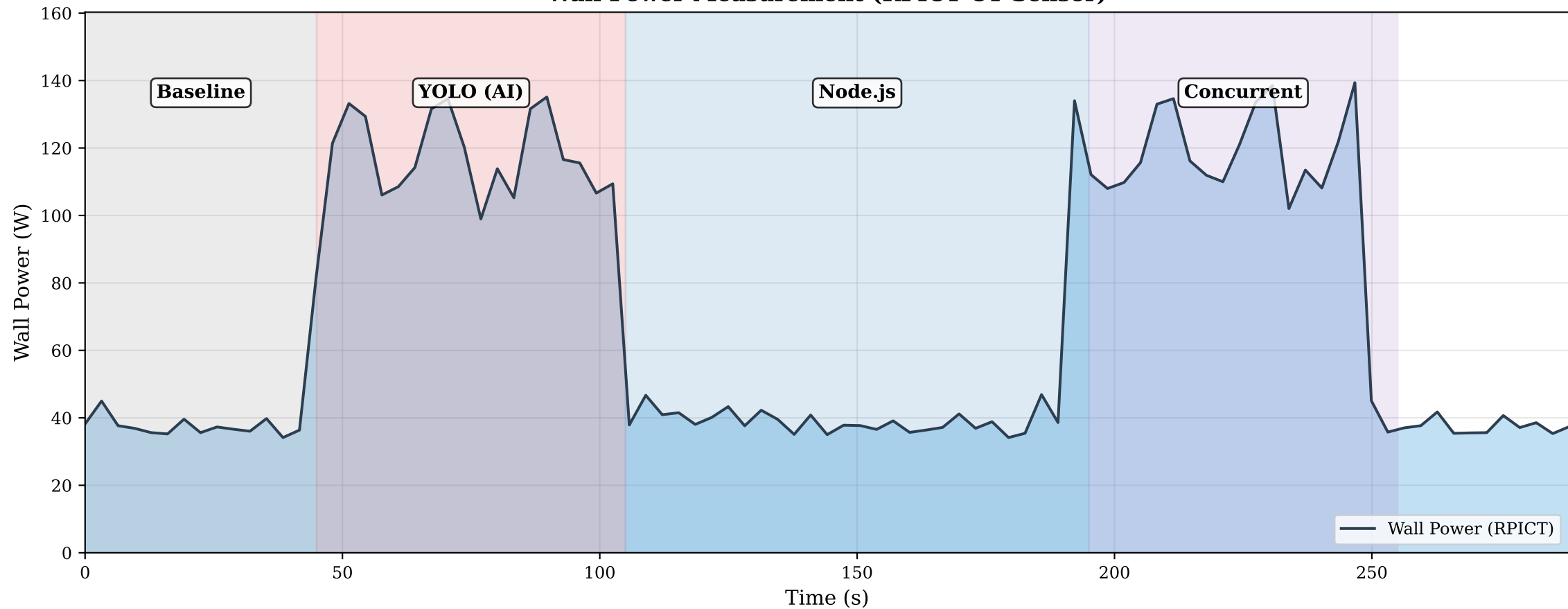
Wall Power Measurement (RPICT CT Sensor)
