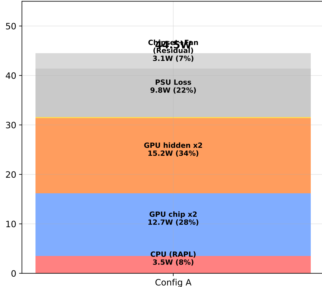
After: Decomposed (Residual 3.1W = 7%)
