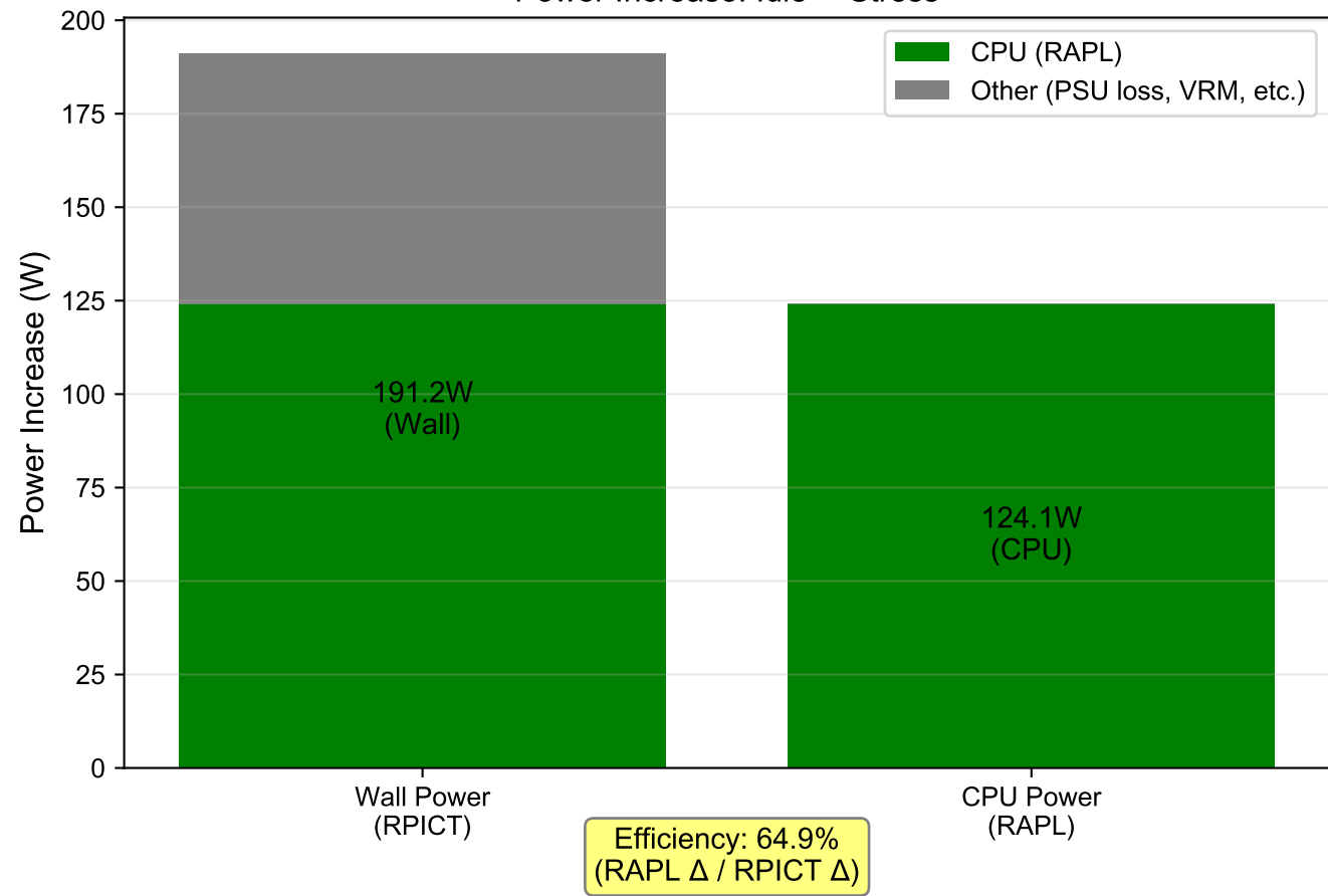
Power Increase: Idle → Stress
