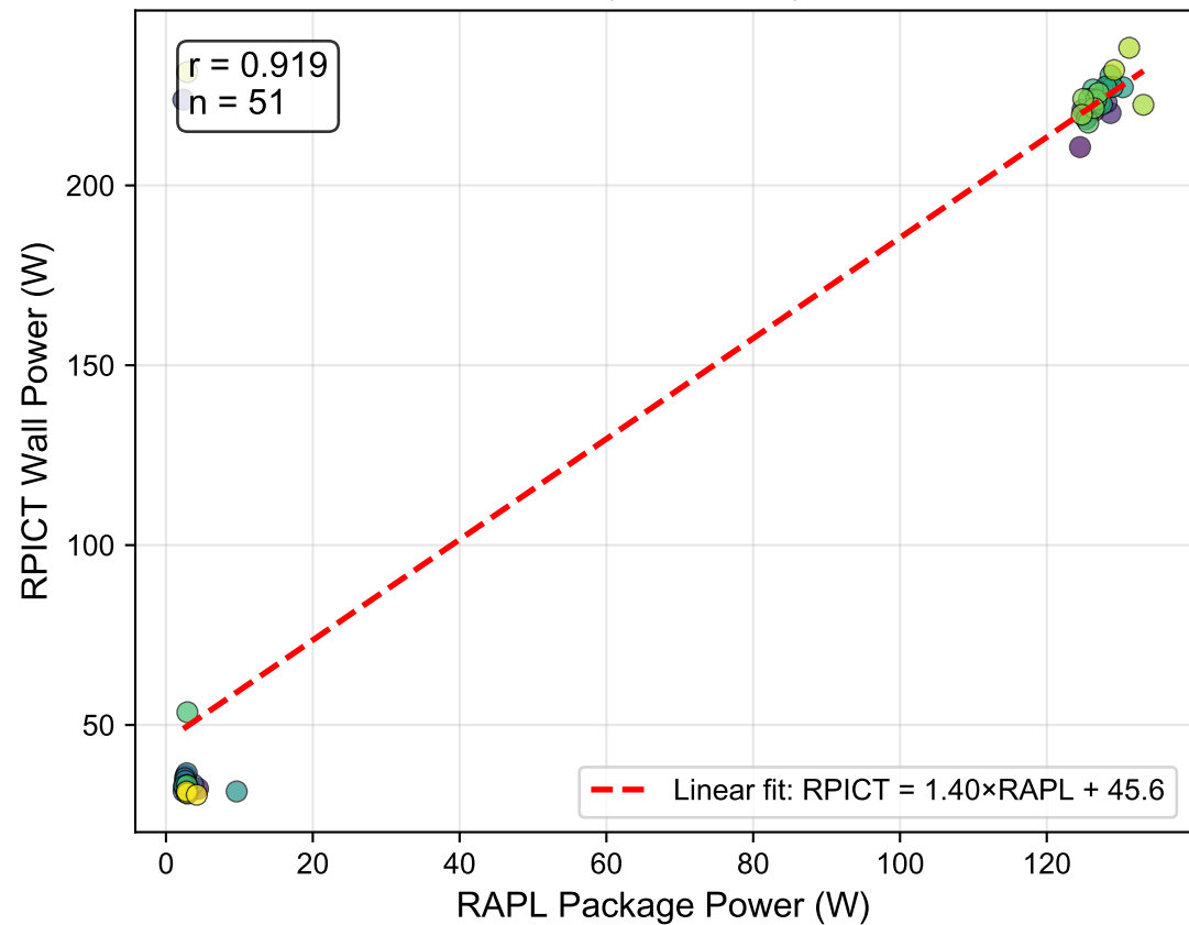
RAPL vs RPICT (Wall Power) Correlation
