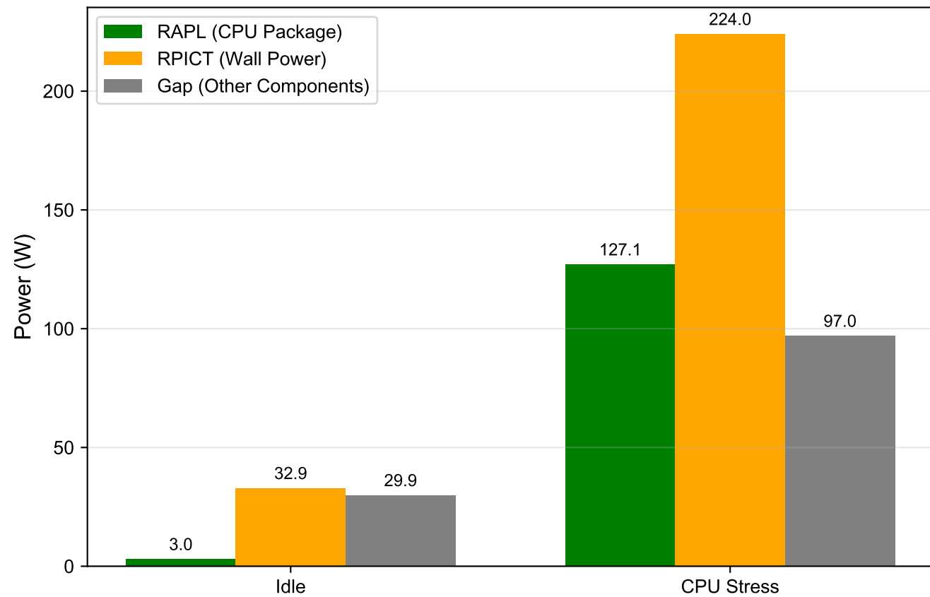
Power Breakdown: RAPL vs Wall Power
