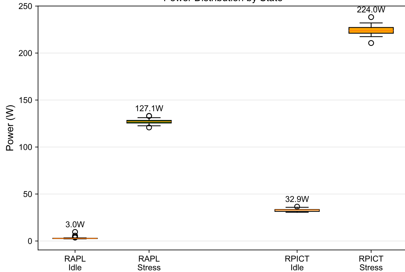
Power Distribution by State
