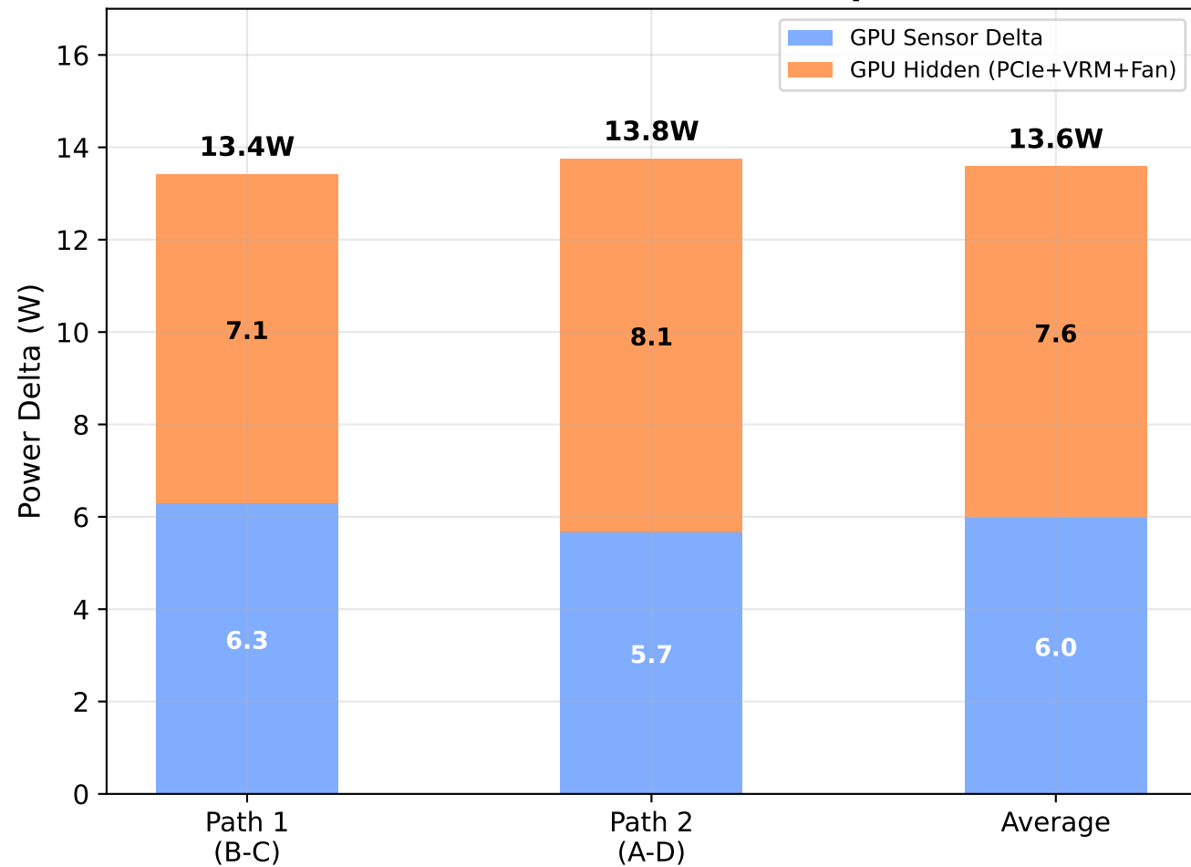
GPU Card: Wall Power Impact
