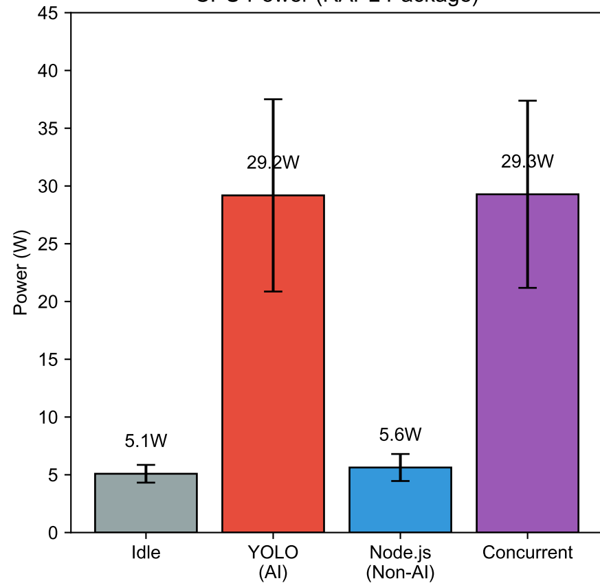
CPU Power (RAPL Package)
