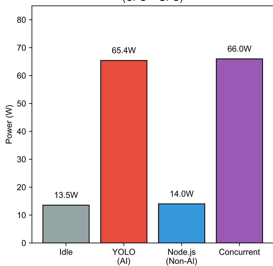
Total Internal Power (CPU + GPU)
