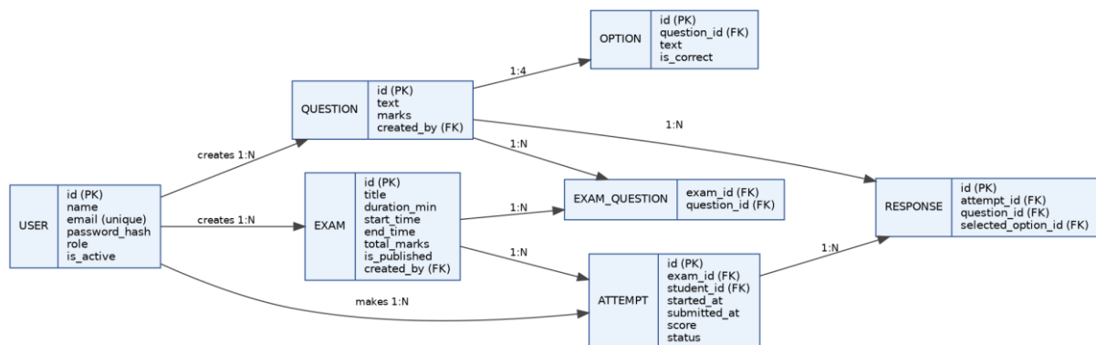
Figure 2: Entity-relationship diagram
