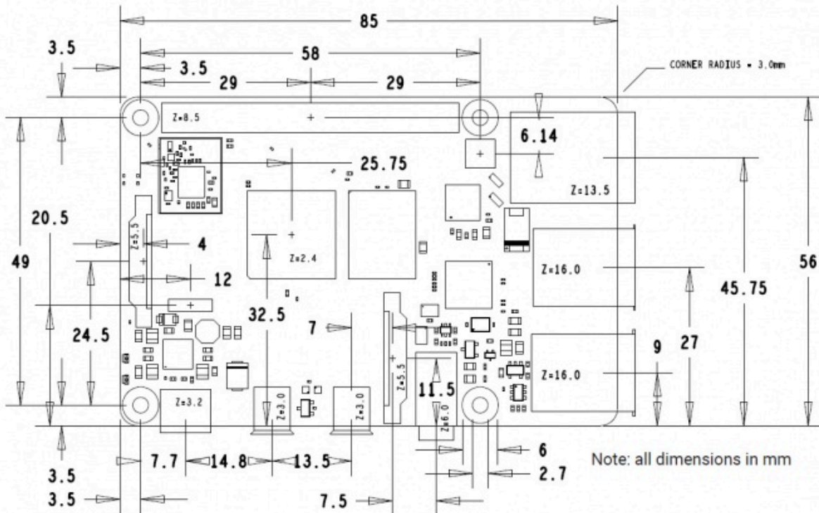
Raspberry pi 4 dimensions
